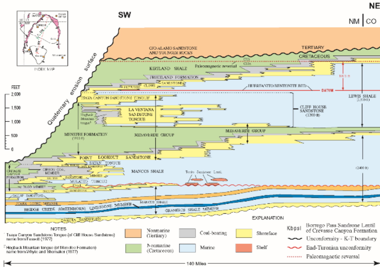
Figure 4. Stratigraphic section showing Upper Cretaceous rocks in the San Juan Basin, New Mexico and Colorado. Tecito Sandstone Lenticle and coal-bearing zones are shown diagrammatically. Stratigraphy of rock units from the Point Lookout Sandstone upward is modified from Fassett (1977), stratigraphy for lower part of section is modified from Nummedal and Molenaar (1995). F - LOS on index map is Fassett (1977) line of cross section; NM - LOS is Nummedal and Molenaar (1995) line of cross section. Position of paleomagnetic reversal from chron C33n to C32r is from Fassett and Steiner (1997). Vertical exaggeration x 55.
