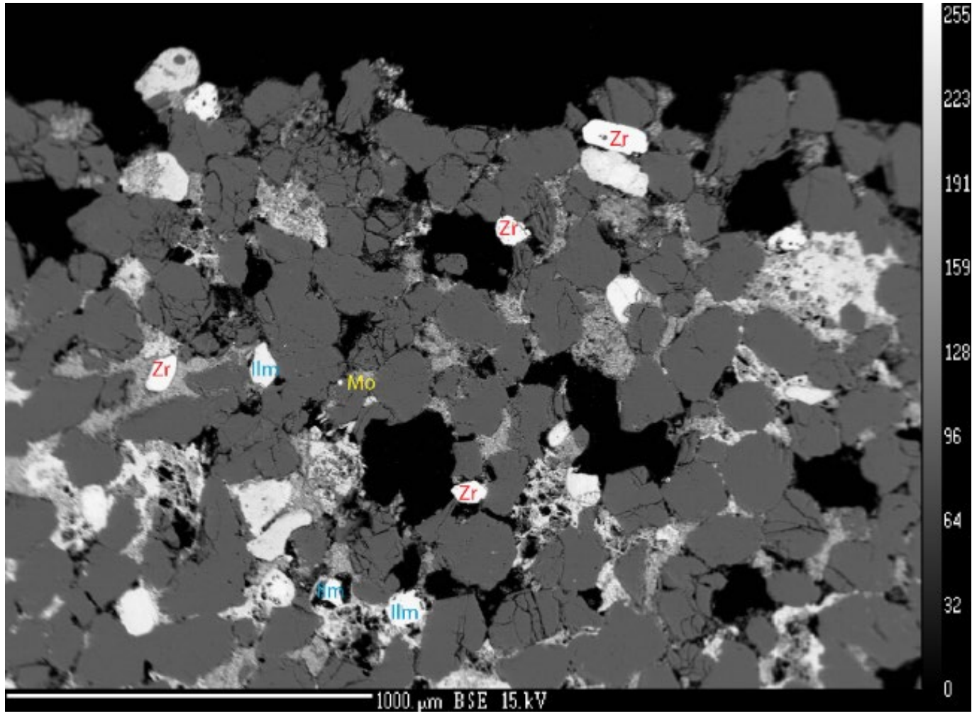
Electron microprobe photo of sample SAN 6 from Sanostee beach-placer deposit Zircon =red, ilmenite =blue, and monazite =yellow (REE mineral), mottled, lighter colored cement=iron oxide (hematite), dark grey grains=quartz, black areas=pore spaces
