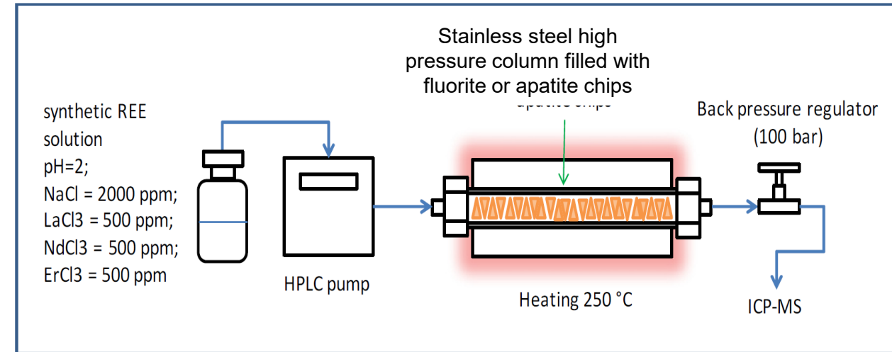
Schematic of separation and extraction hydrothermal reactor proof-of-concept experiments
