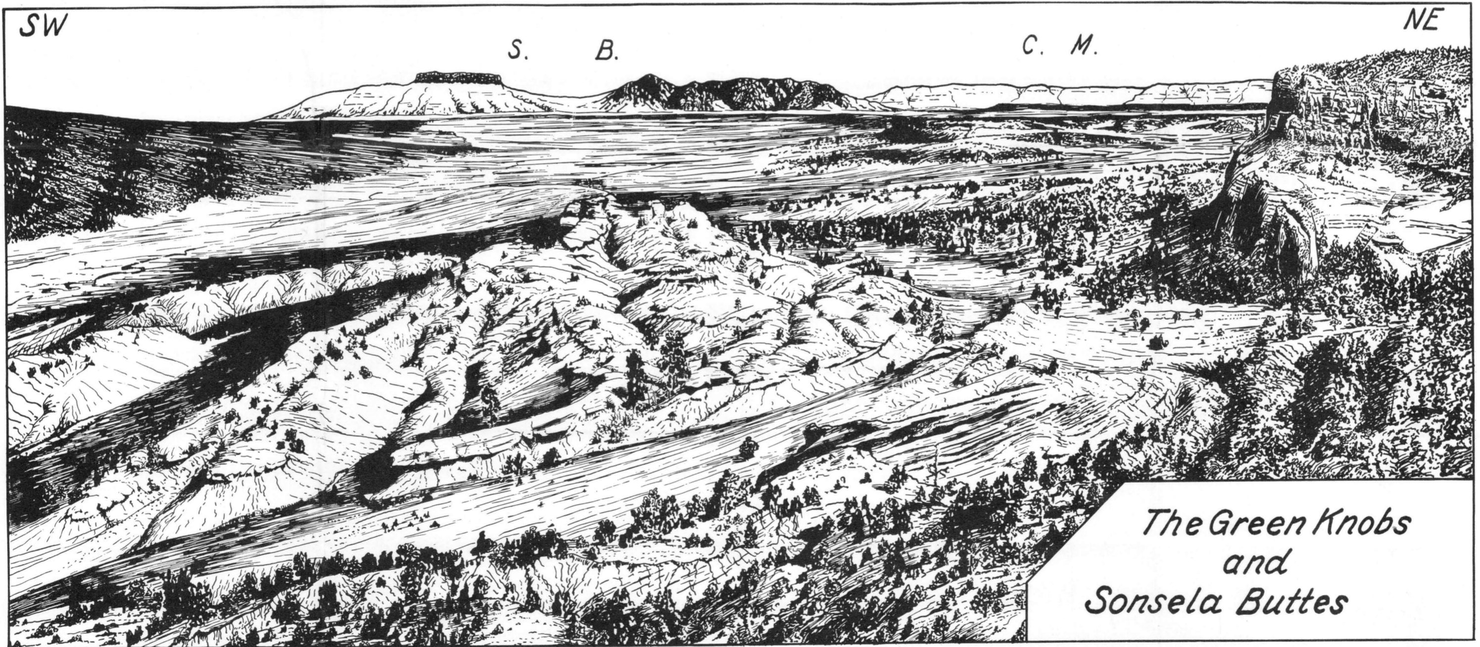
B. View across Green Knobs from the southeast. Light-colored cliffs are pale-green lapilli tuff, showing flat layers near center and progressively steeper dips along southeastern contact (foreground). Forested cliffs on right are Entrada and Summerville formations (west border of Todilto Park) resting on Chinle shales that underline flat plain in middle distance. Lower Chinle sandstones, rising toward Defiance uplift, form forested slope near left margin. Sonsela Buttes (S.B.), consisting of plugs and short flows of minette and trachybasalt, and Chuska Mountain (C.M.) on skyline.
