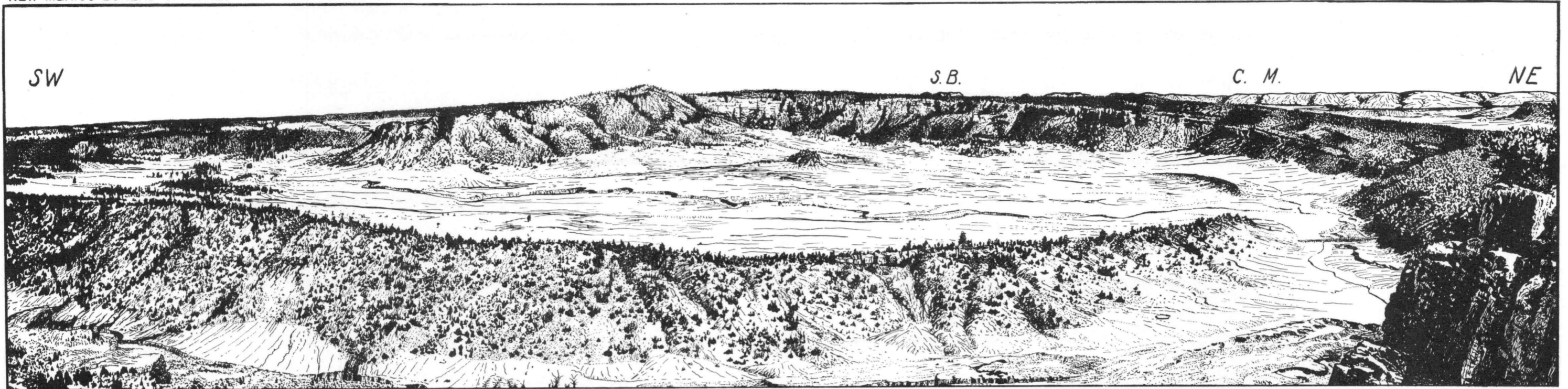
A. View across Buell Park from the southeast. Flat plain underlain by lapilli tuff with discontinuous cover of alluvium. Hill of kimberlite tuff near center of plain. Minette ring-dike, breached by Buell Creek, forms ridge in foreground and near right edge of plain. Buell Mountain, in left distance, is a complex of minette dikes and plugs of trachytic phases of minette, piercing lapilli tuff. Trachybasalt masses near summit may have approached surface of eruption. Rim rocks are upper Cutler sandstone overlain on right side by De Chelly sandstone, Shinarump conglomerate, and lower Chinle shales. Cliff in right foreground is top of De Chelly sandstone. Sonsela Buttes (S.B.) and Chuska Mountain (C.M.) on skyline.
