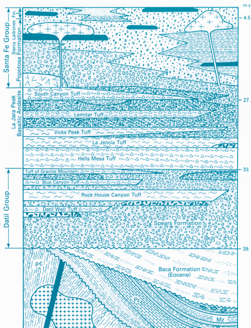
Generalized stratigraphic column for the northeast Mogollon–Datil volcanic field, New Mexico
