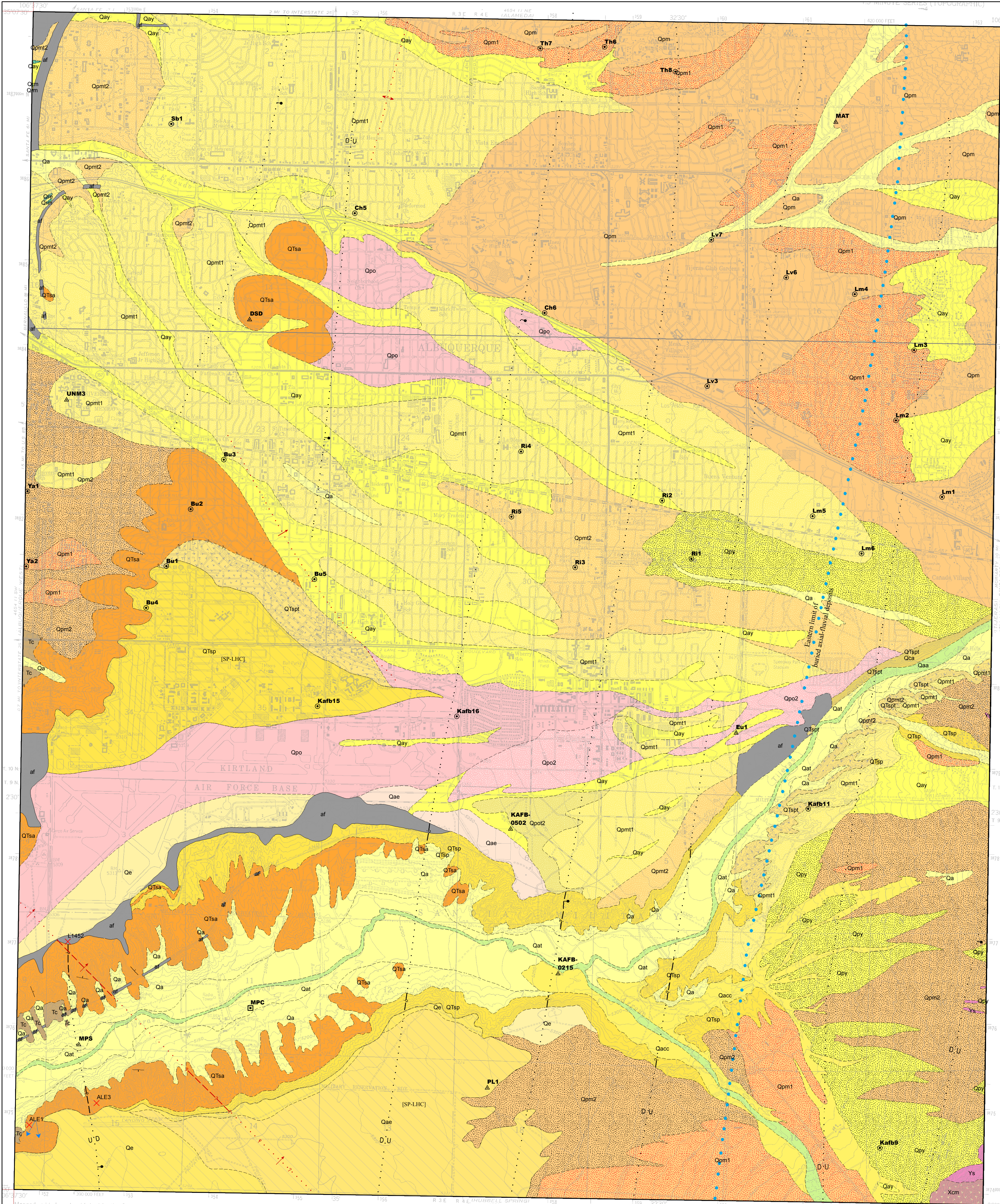
Geologic Map of the Albuquerque East 7.5-Minute Quadrangle, Bernalillo County, New Mexico by Hawley, J.; Chamberlin, R. M.; Connell, S. D. Scale: 1:24,000
