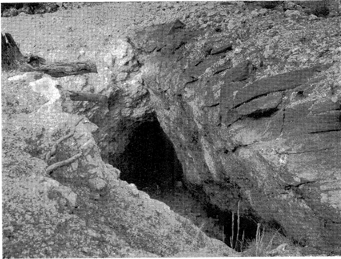
Stoped portion of mica-bearing hanging-wall zone in Queen deposit, looking west and down. This is a part of south arm of plunging trough-like pegmatite body. Note gentle rolls in hanging-wall contact; these plunge moderately west-northwest in conformity with entire body.
