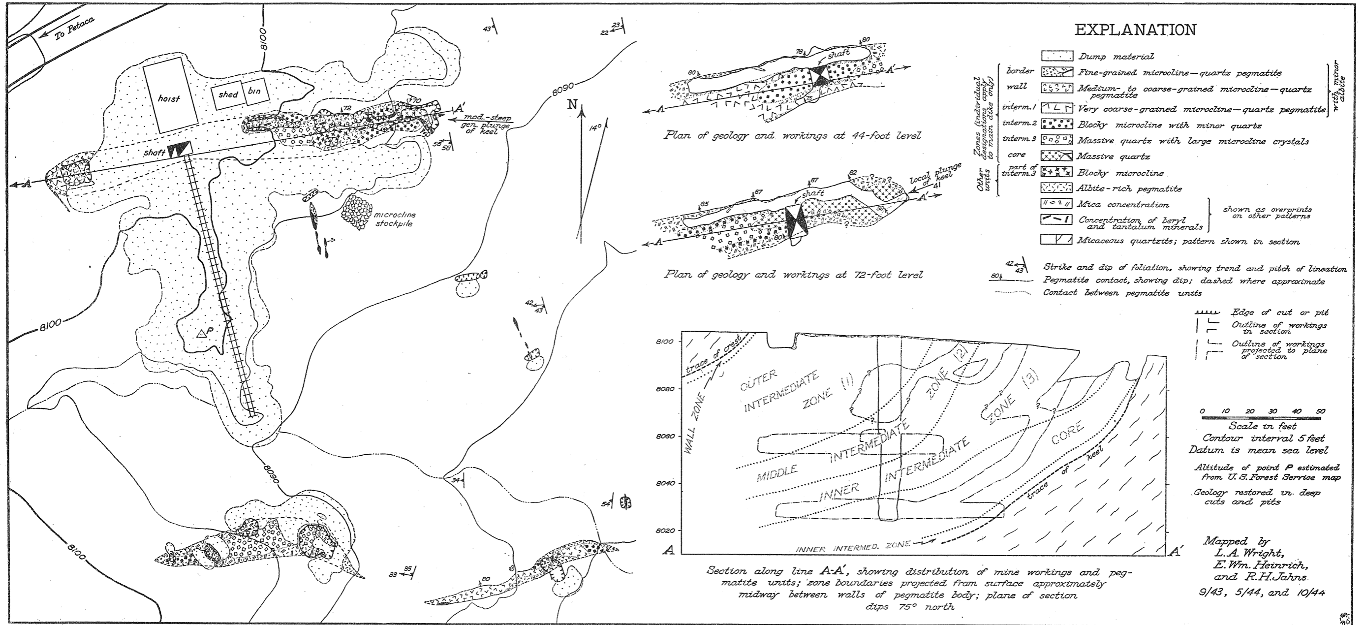
Geologic map, plans, and longitudinal section of the Lonesome deposit.
