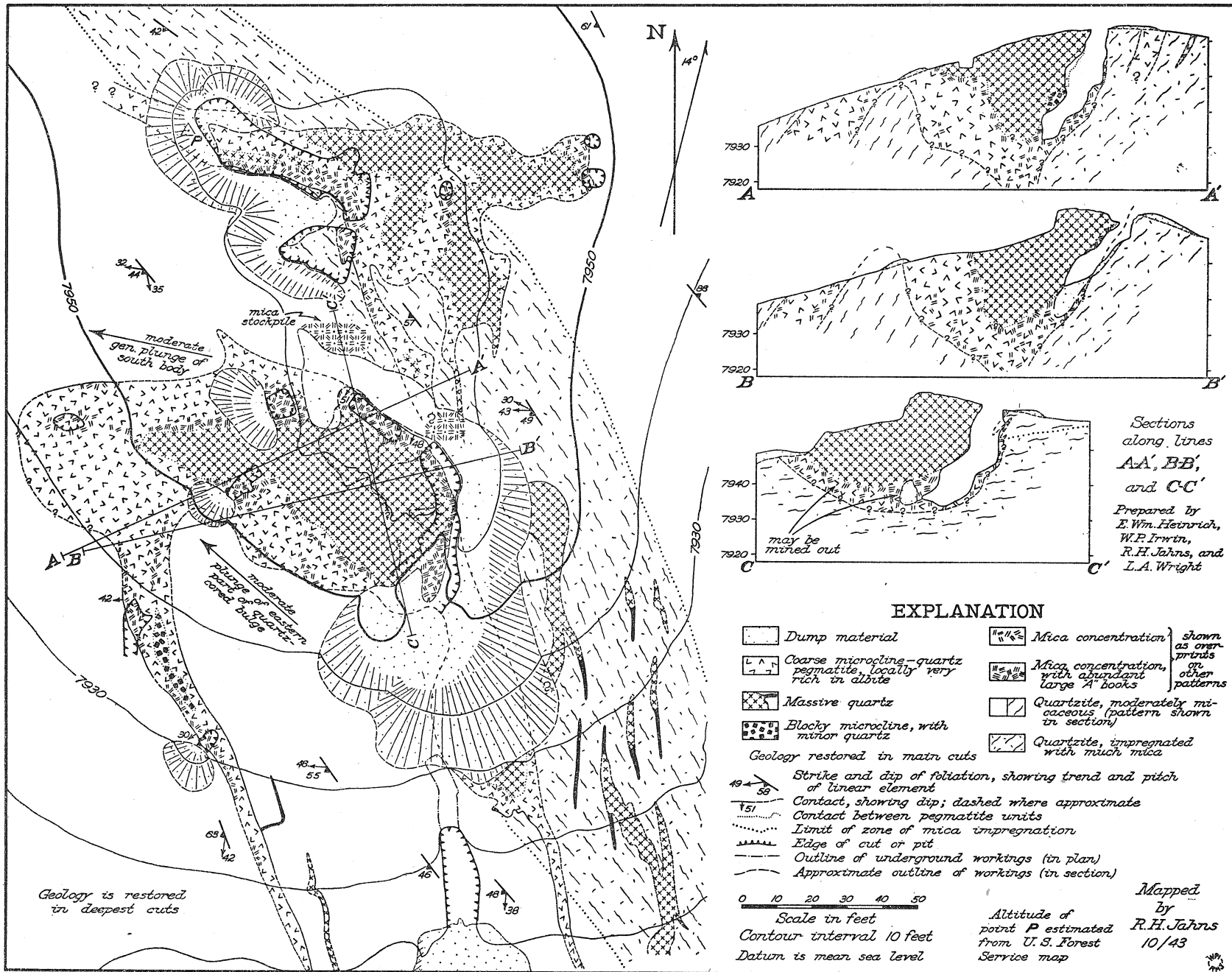
Geologic map and sections of a part of the Sandoval deposit.
