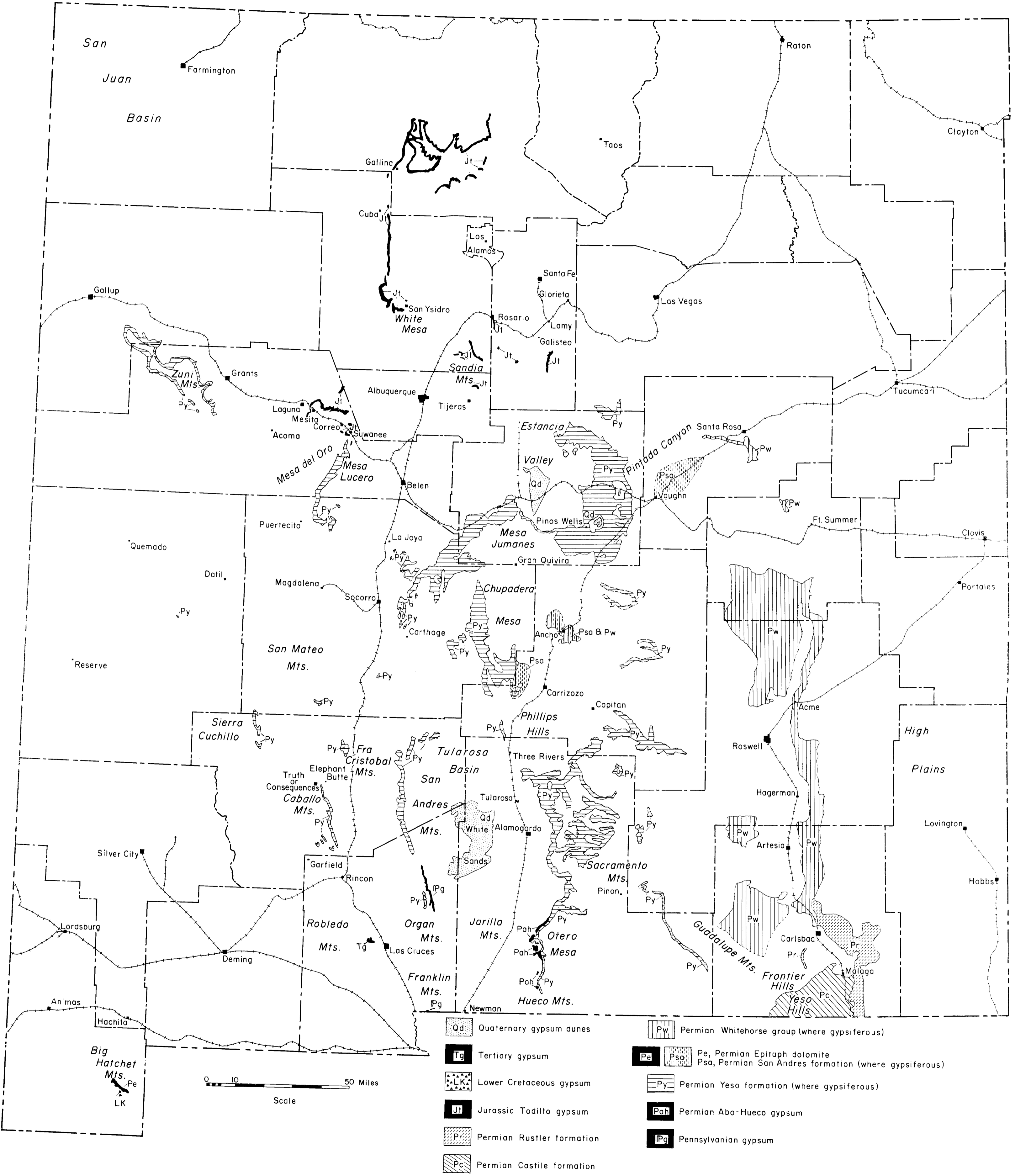
INDEX MAP OF GYPSUM DEPOSITS IN NEW MEXICO
