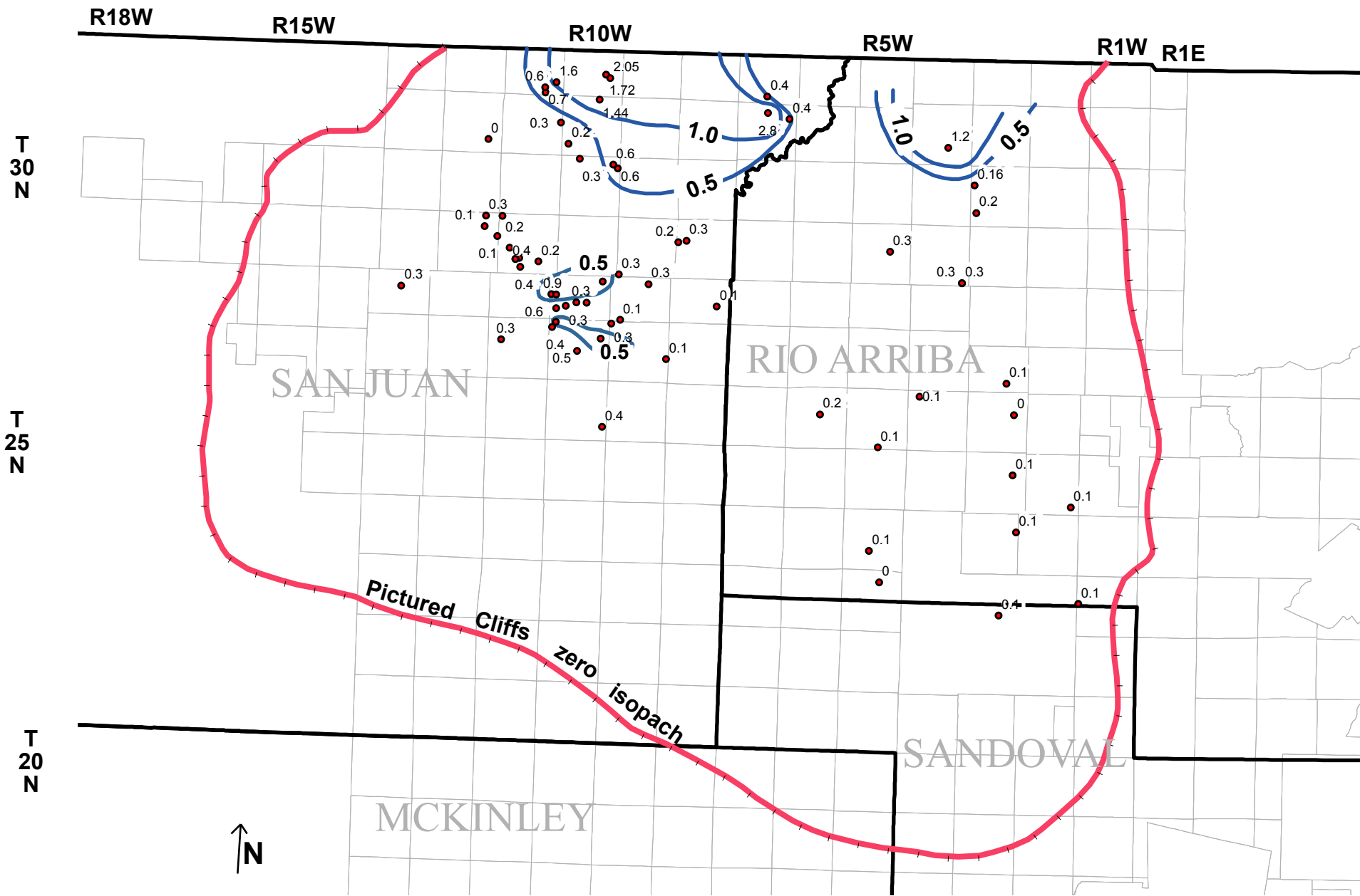
Contours in mole percent CO 2 in Pictured Cliffs gases
