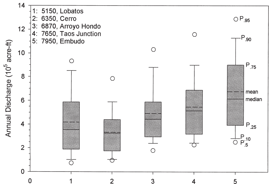
FIGURE 4—Variability of annual discharge for Rio Grande gage stations.
