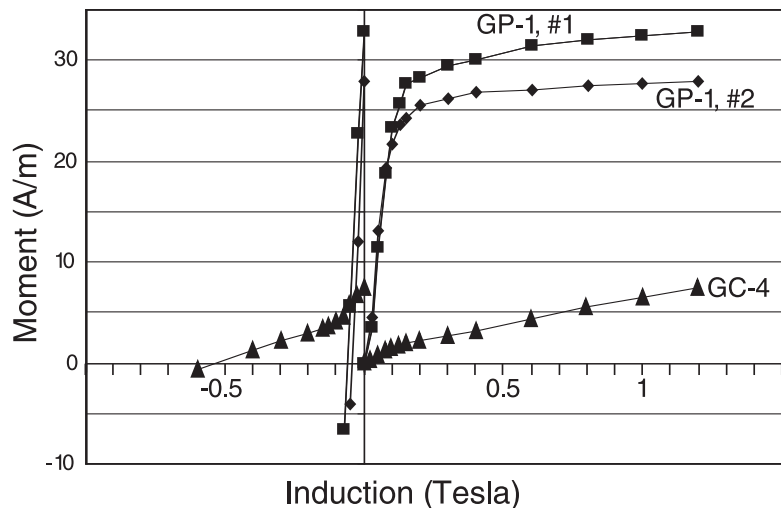
FIGURE 5—Acquisition of isothermal remanent magnetization of Grober-Fuqua #1 well core samples. Backfield demagnetization of remanence acquired at 1.2 T gives coercivity of remanence values that are indicative of hematite for the GC-4 horizon (triangles) and magnetite for the GP-1 horizon (squares and diamonds).
