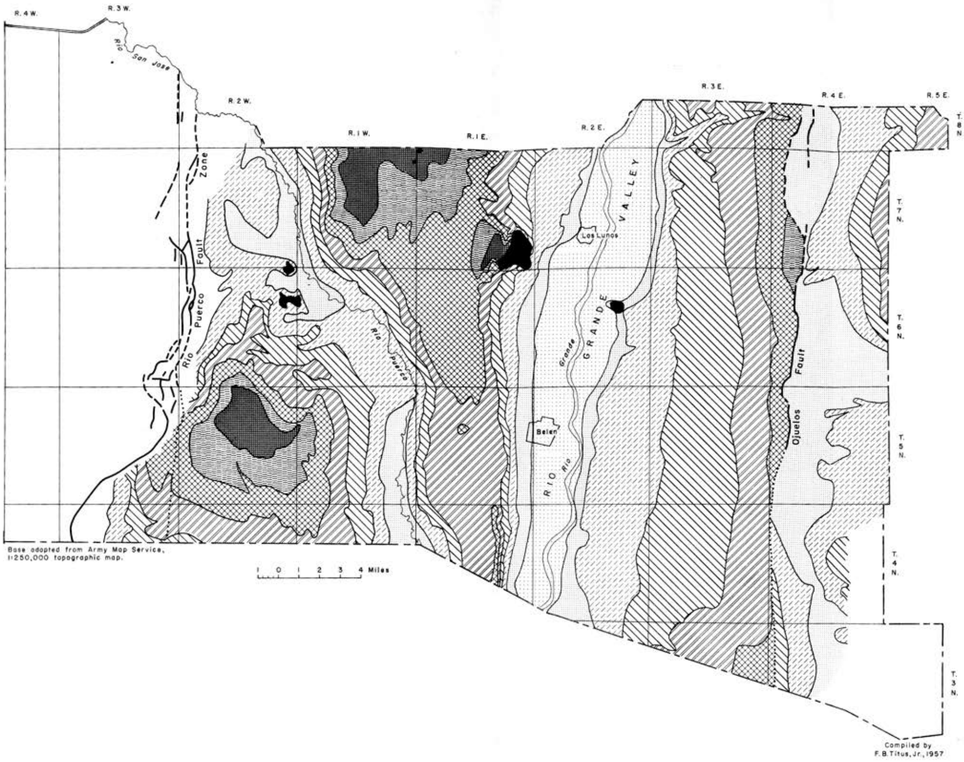
Plate 2 DEPTH-TO-WATER MAP FOR THE RIO GRANDE GRABEN IN VALENCIA COUNTY, N. MEX.
