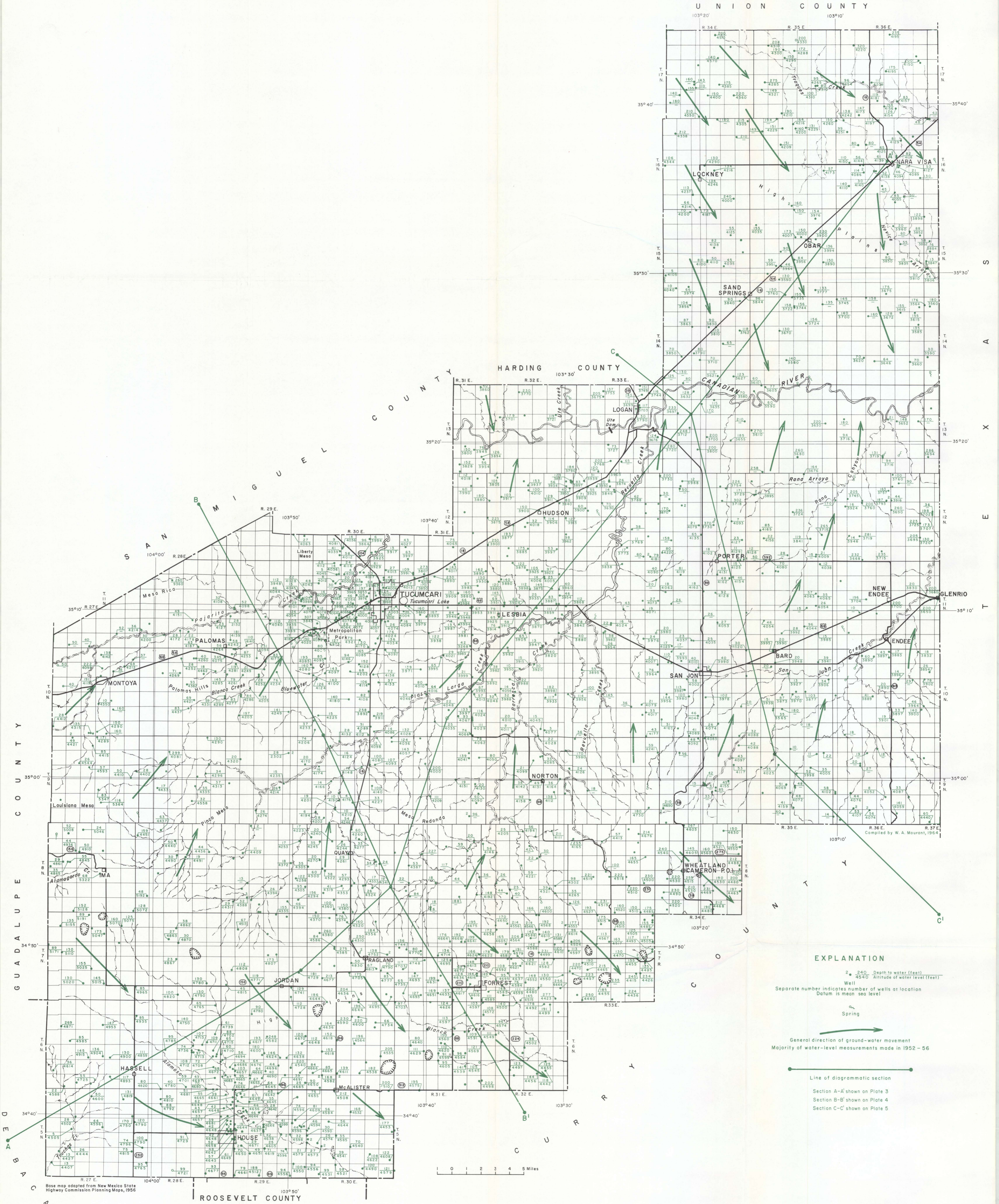
LOCATION OF SELECTED WELLS IN QUAY AND ADJOINING COUNTIES, NEW MEXICO AND GENERAL DIRECTION OF GROUND-WATER MOVEMENT
