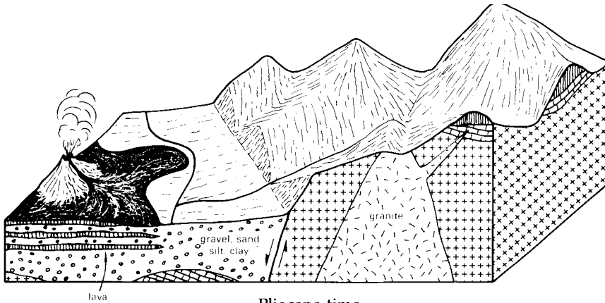
Pliocene time. Continuing uplift and settling; erosion in the mountains; rift-basin sediments and lava cover plain.
