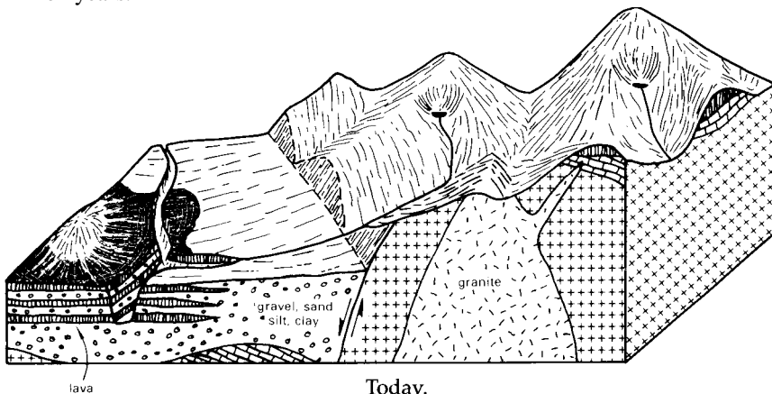
Today. Mountains, plain, and gorge; lakes high in the mountains are where glaciers scoured out depressions.
