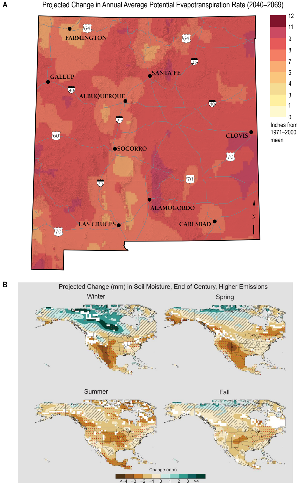
Figure 2.6. (A) Projected change in annual rate of potential evapotranspiration (inches from 1971–2000 mean), derived from the same projections used for Figures 2.1B and 2.3. (B) Projected changes in seasonal soil moisture by the end of the twenty-first century across North America, adapted from USGCRP (2017).
