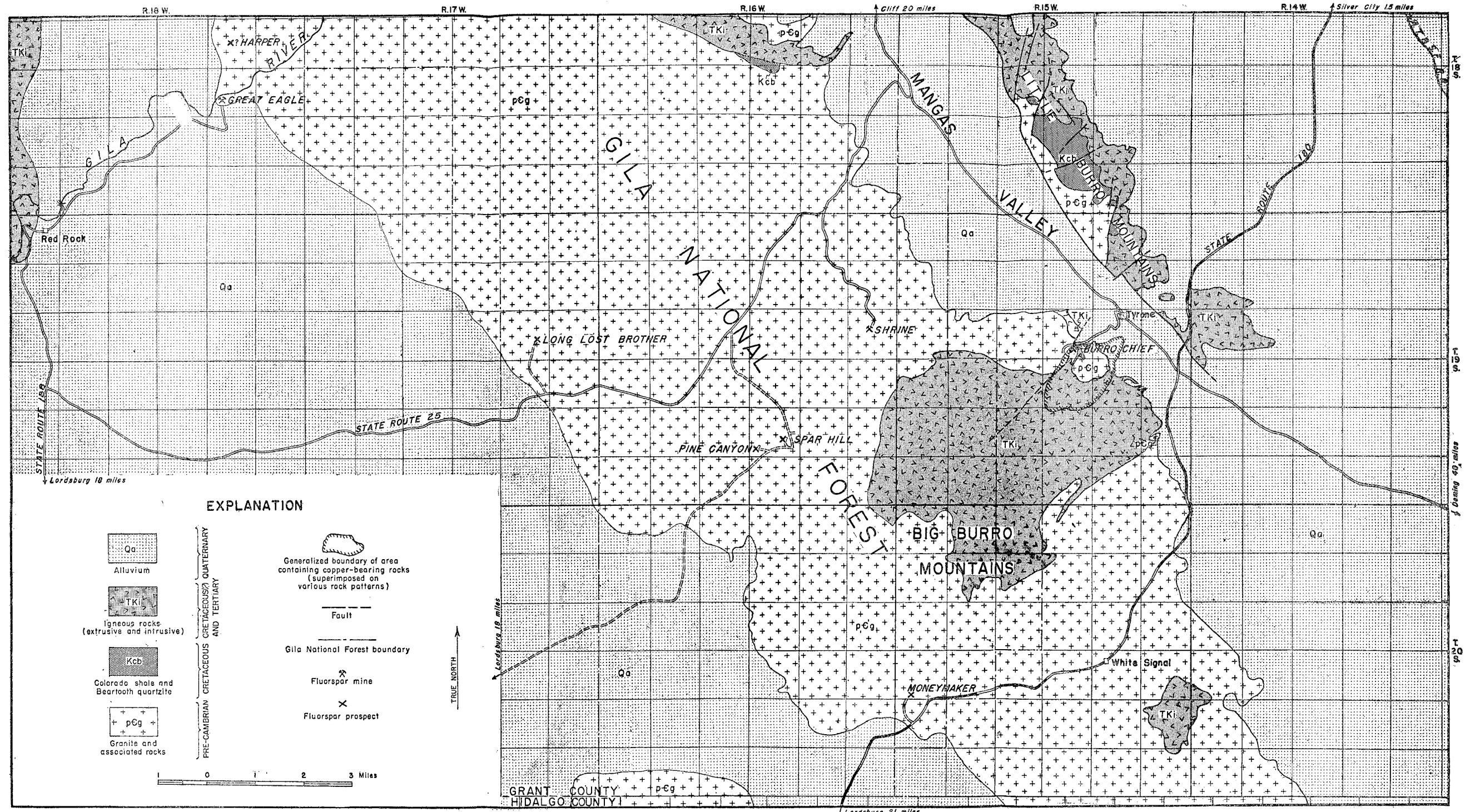
Generalized geologic map of the Burro Mountains and vicinity, Grant County, showing location of fluspar deposits
