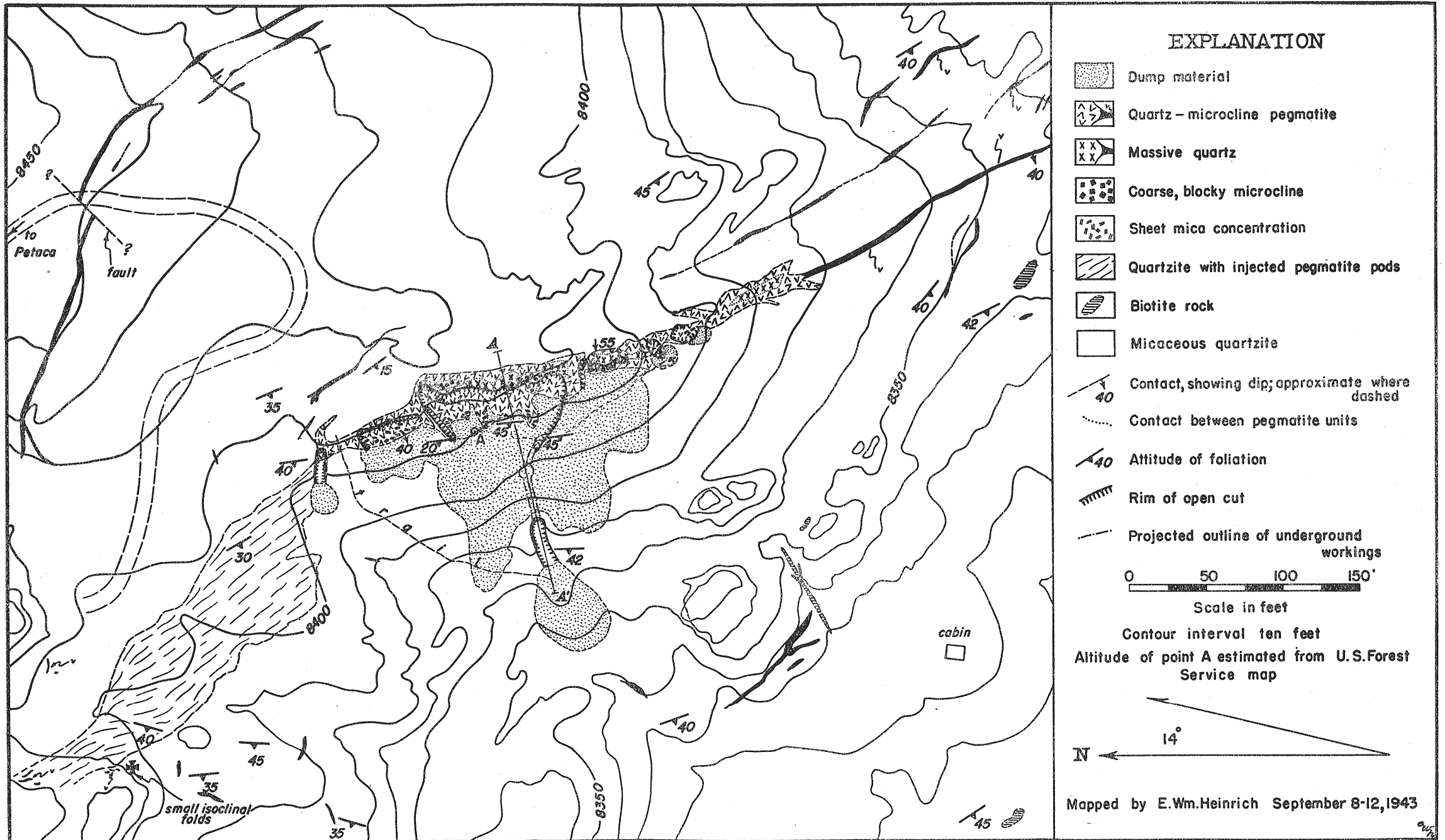
Geologic map of the Alma deposit (see FIGURE 10 for cross section).
