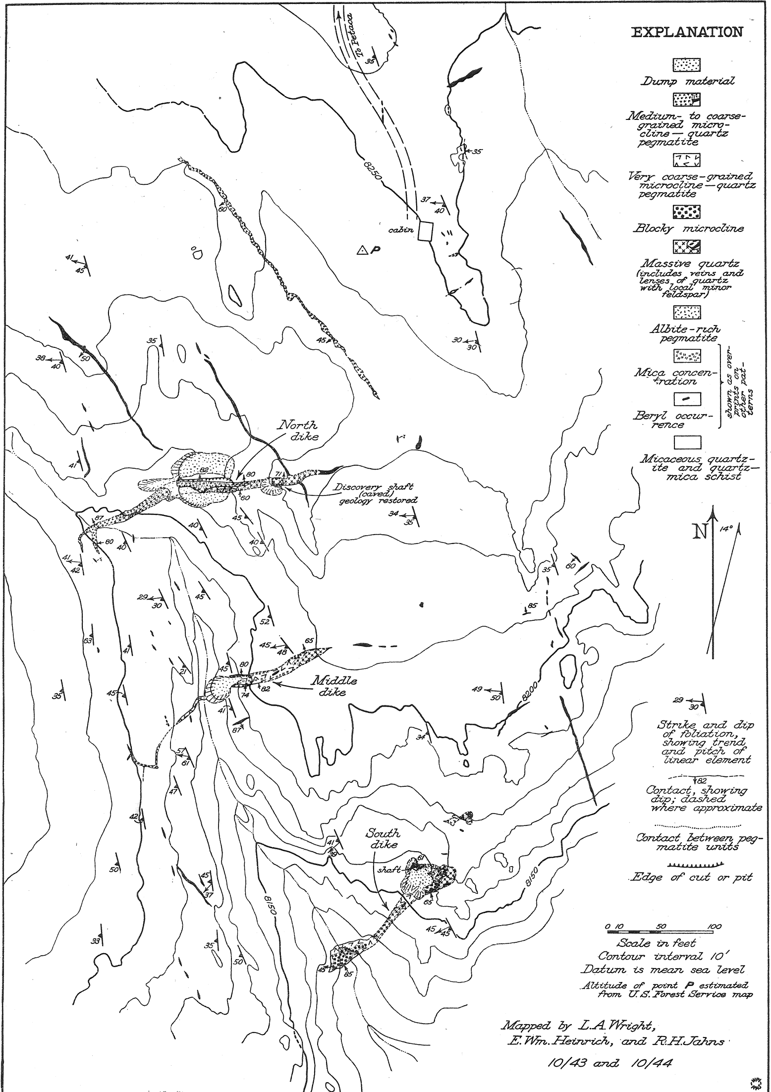
Geologic map of the La Jarita deposit.
