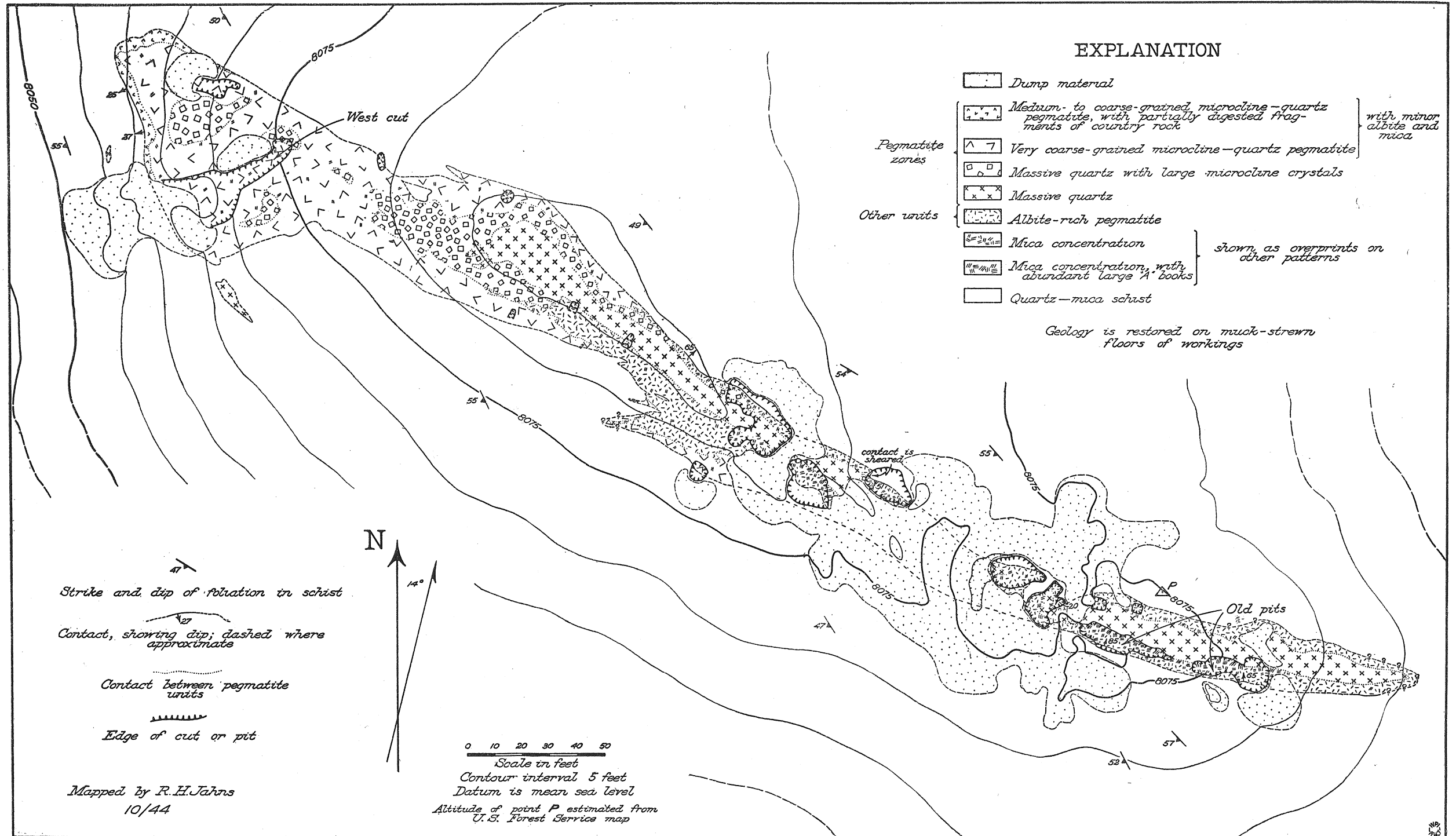
Geologic map of the North Star deposit.
