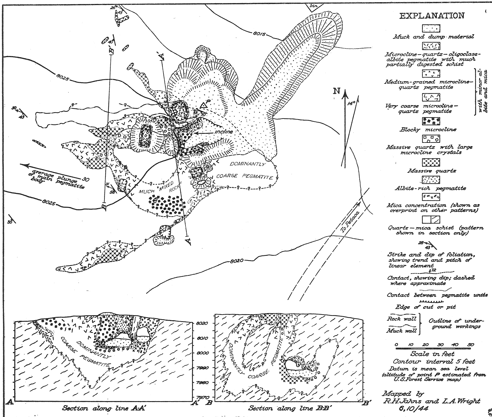
Geologic map and sections of the Conquistador deposit.
