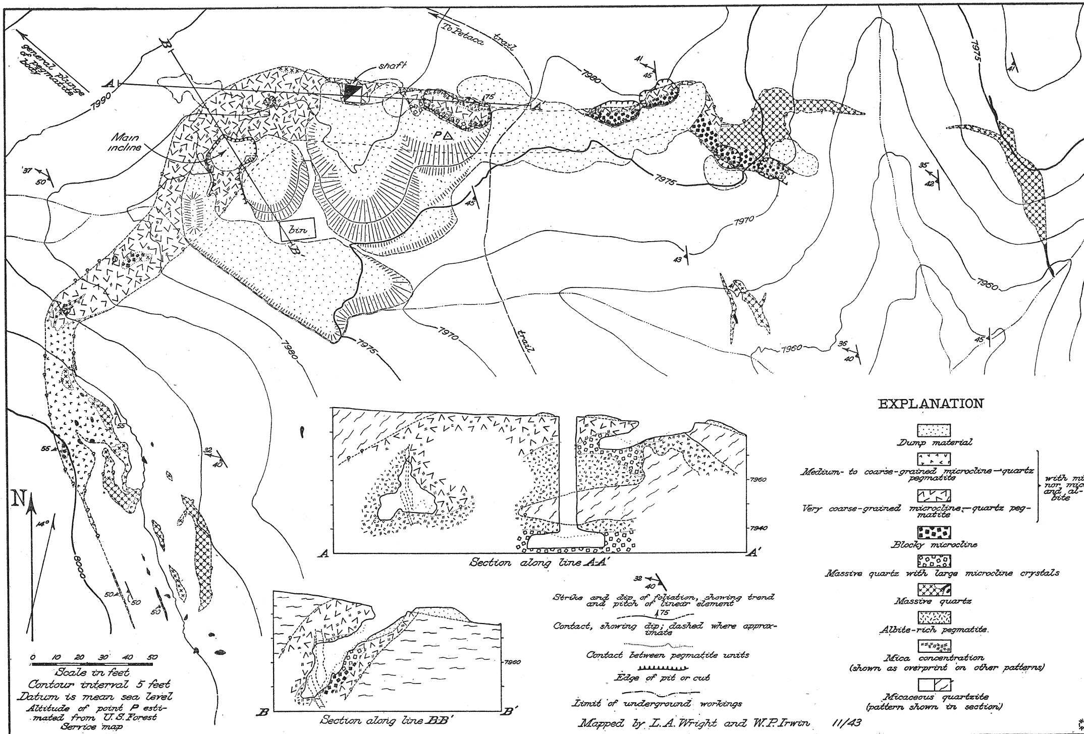
Geologic map and sections of the Keystone-Western deposit.
