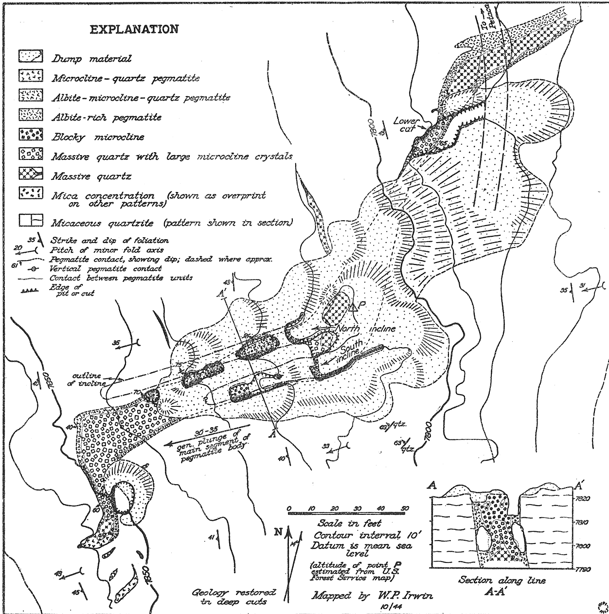
Geologic map and section of the Pinos Altos deposit.
