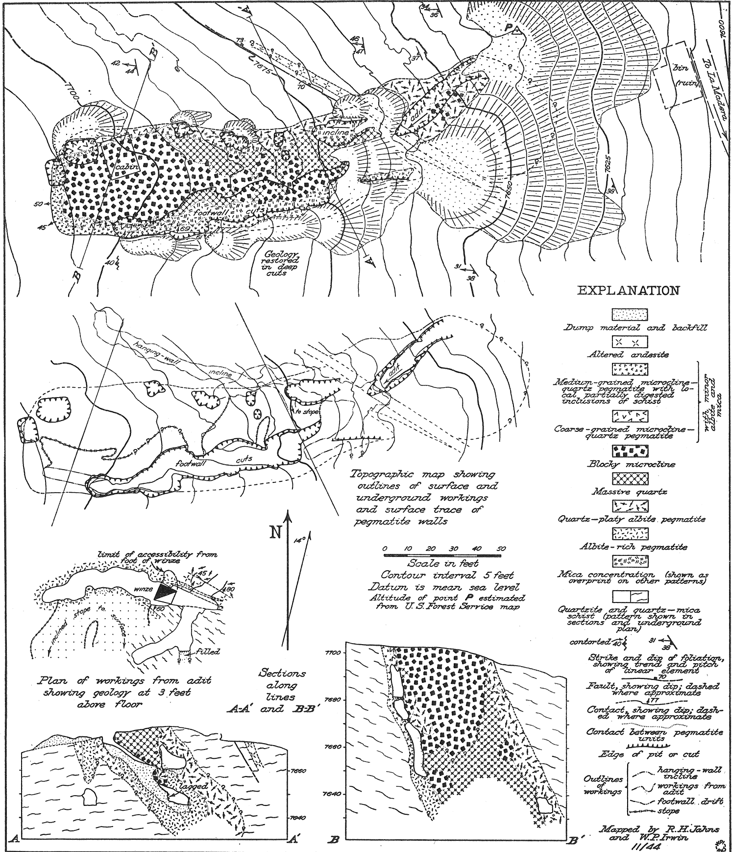
Geologic map, plans, and sections of the White deposit.
