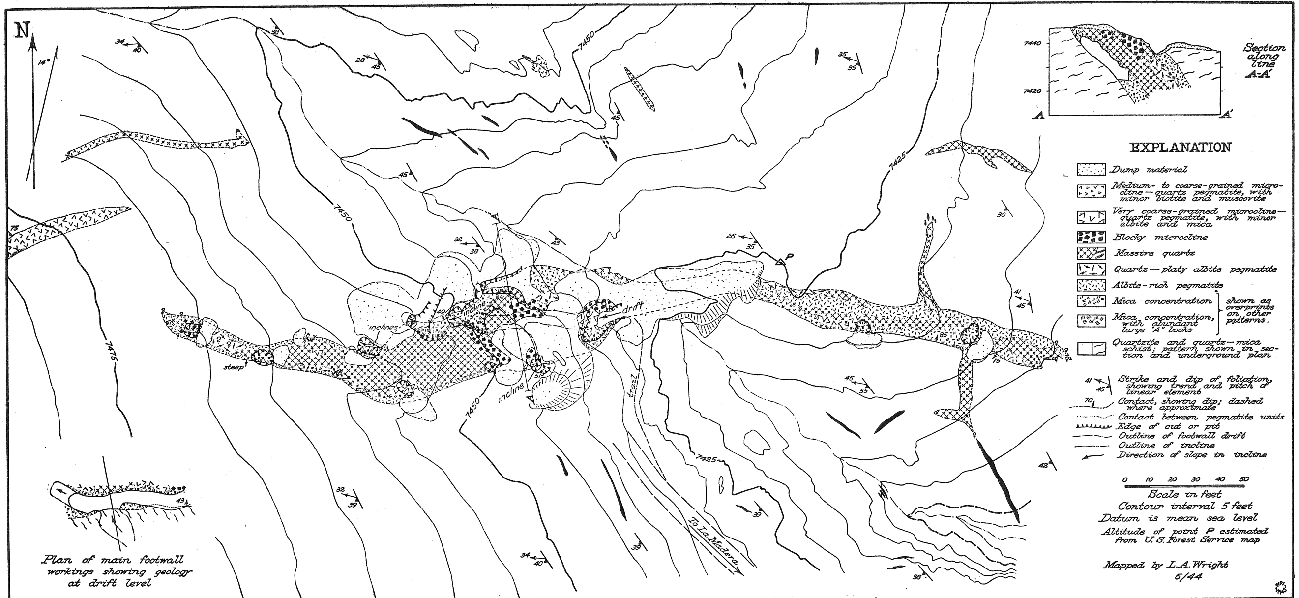
Geologic map, plan, and section of the Hidden Treasure deposit.
