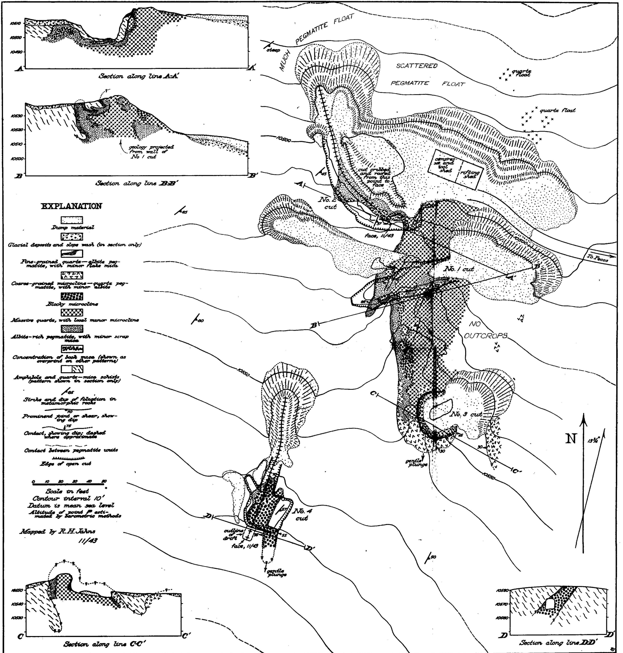
Geologic map and sections of the Elk Mountain deposit. Reference point P is in foundation at north corner of compressor and tool shed. NEW MEXICO BUREAU OF MINES AND MINERAL RESOURCES, SOCORRO, NEW MEXICO
