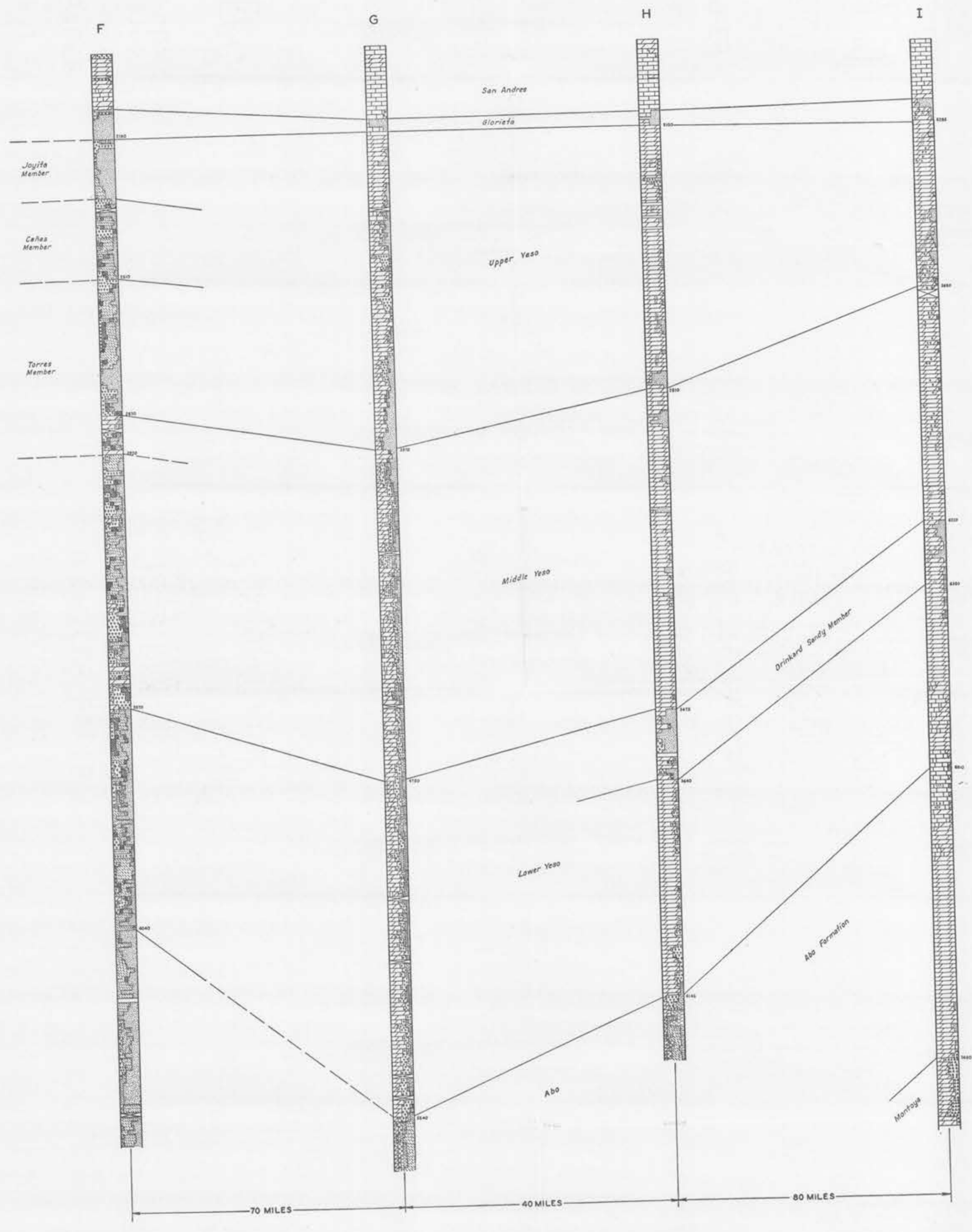
COMPARATIVE SECTIONS OF YESO FORMATION IN SELECTED WELLS
