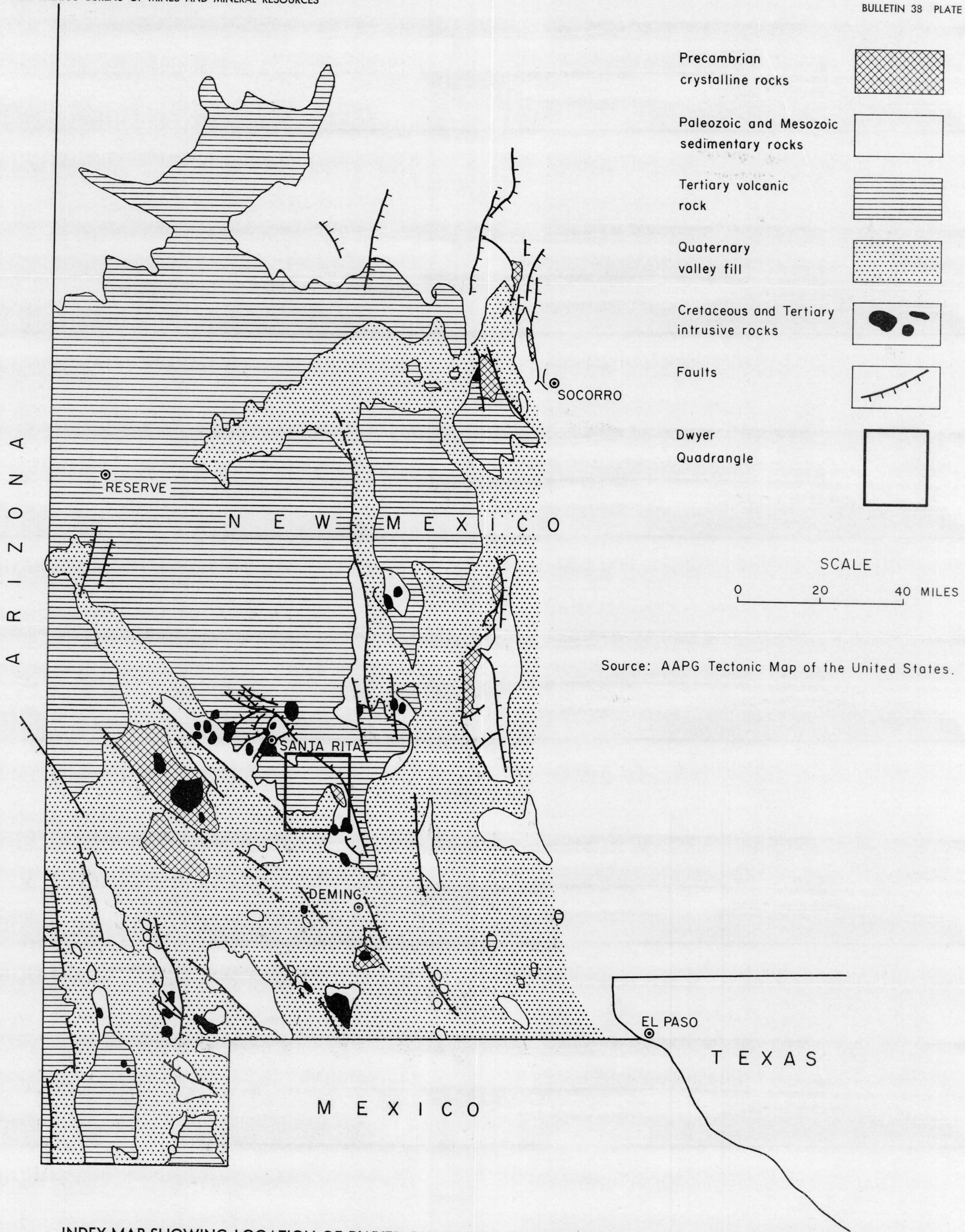
INDEX MAP SHOWING LOCATION OF DWYER QUADRANGLE AND ITS SETTING IN THE REGIONAL GEOLOGY OF SOUTHWESTERN NEW MEXICO
