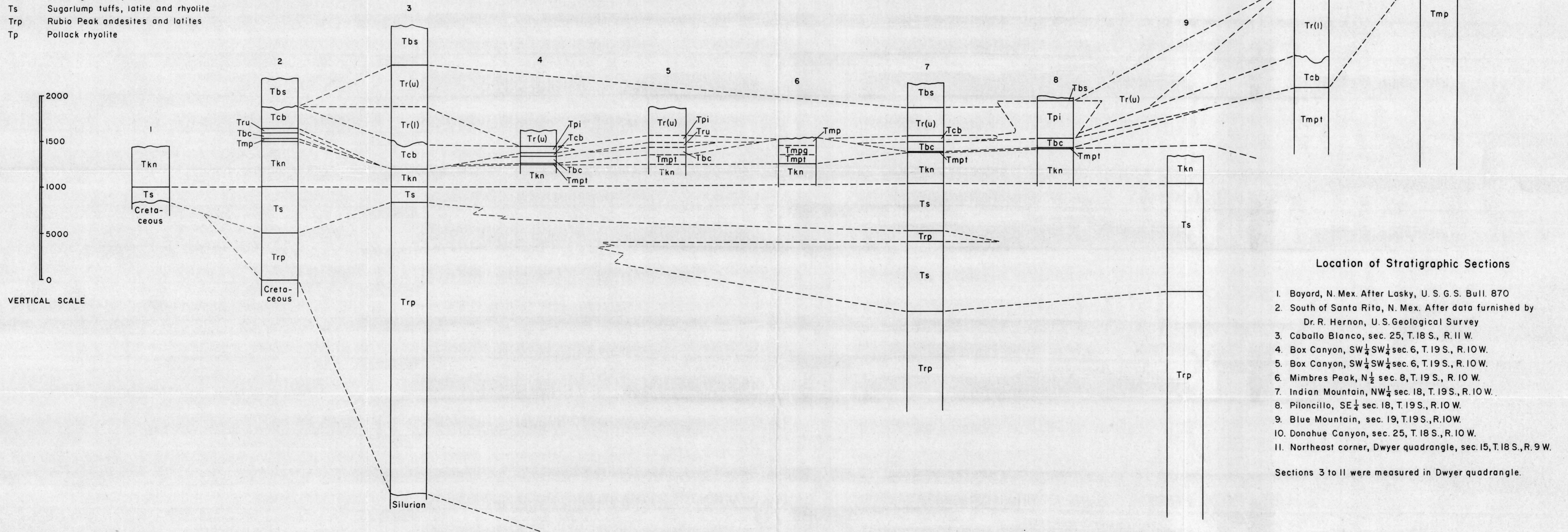
COMPARATIVE TERTIARY STRATIGRAPHIC SECTIONS OF DWYER QUADRANGLE AND ADJACENT AREAS
