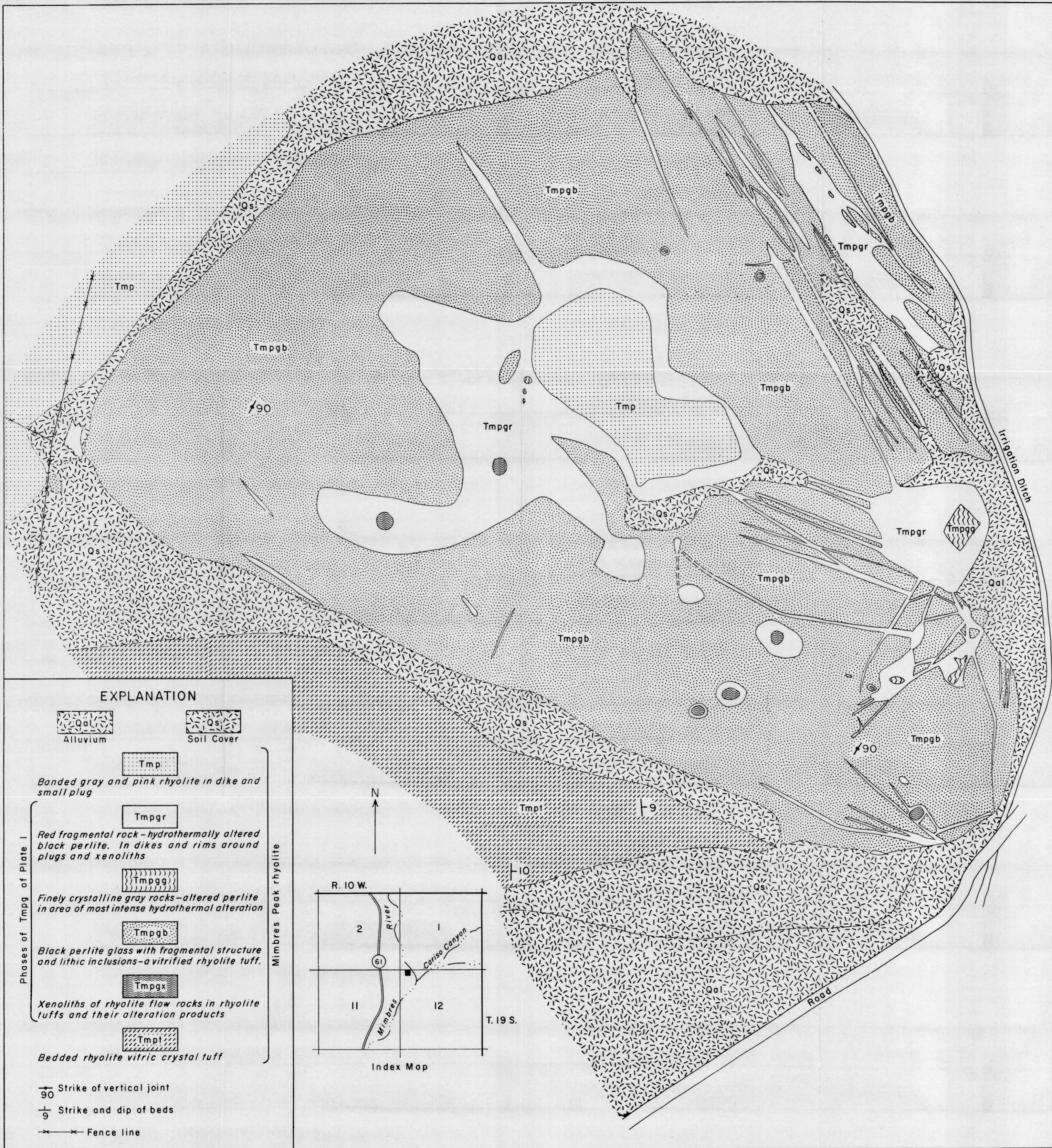
HYDROTHERMAL ALTERATION OF PERLITIC RHYOLITE GLASS
