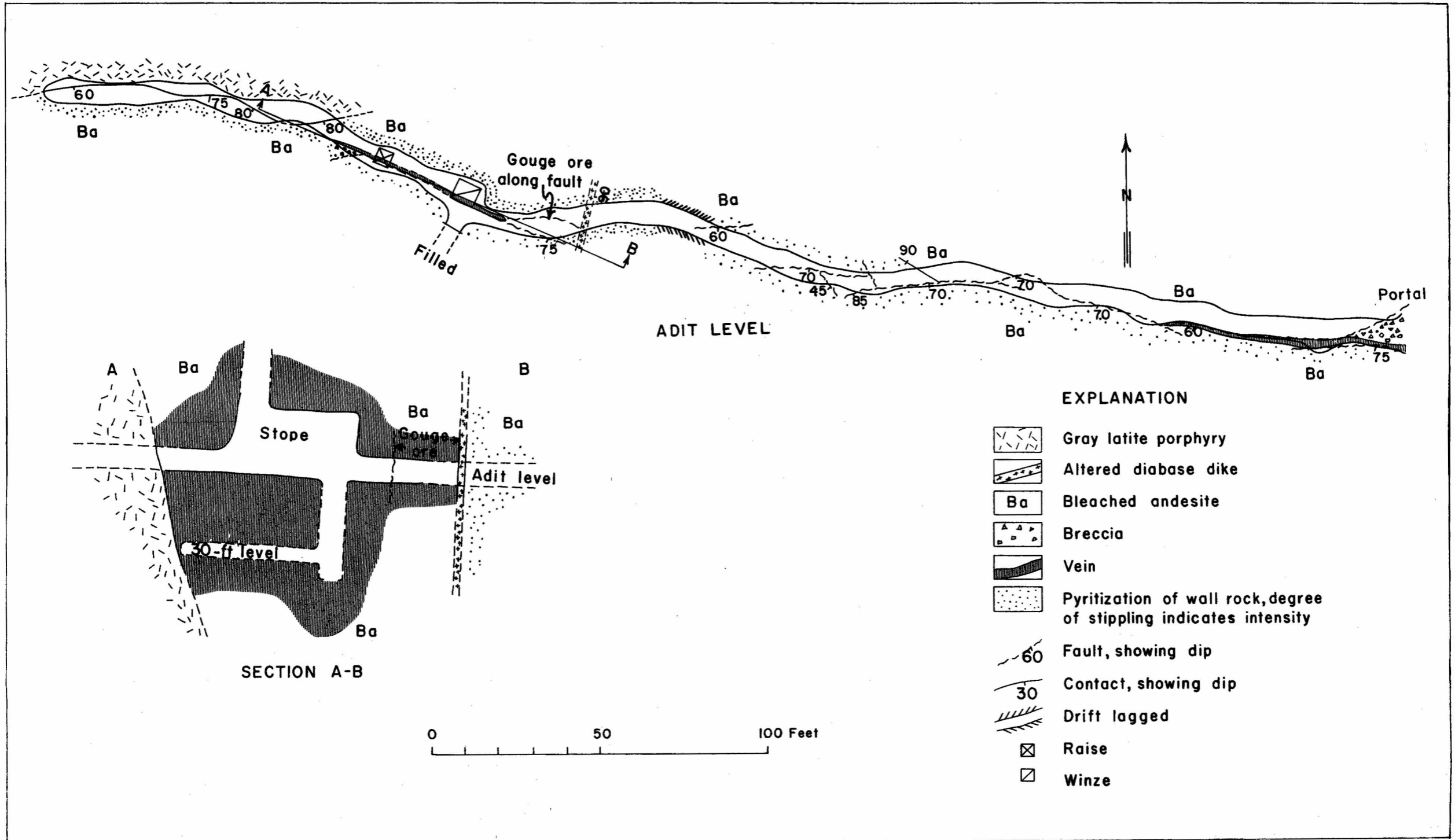
GEOLOGIC MAP AND SECTION OF THE RENOWNED MINE (GEOLOGY BY GEORGE B. GRISWOLD, 1958)
