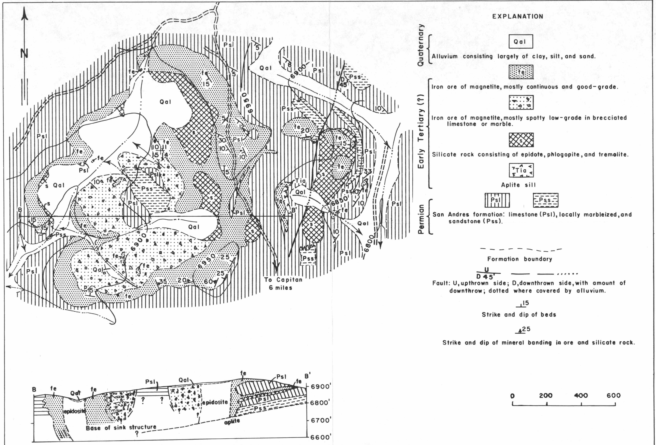
GEOLOGIC MAP OF THE MAIN CAPITAN IRON ORE DEPOSITS (GEOLOGY BY V. C. KELLEY, 1949)
