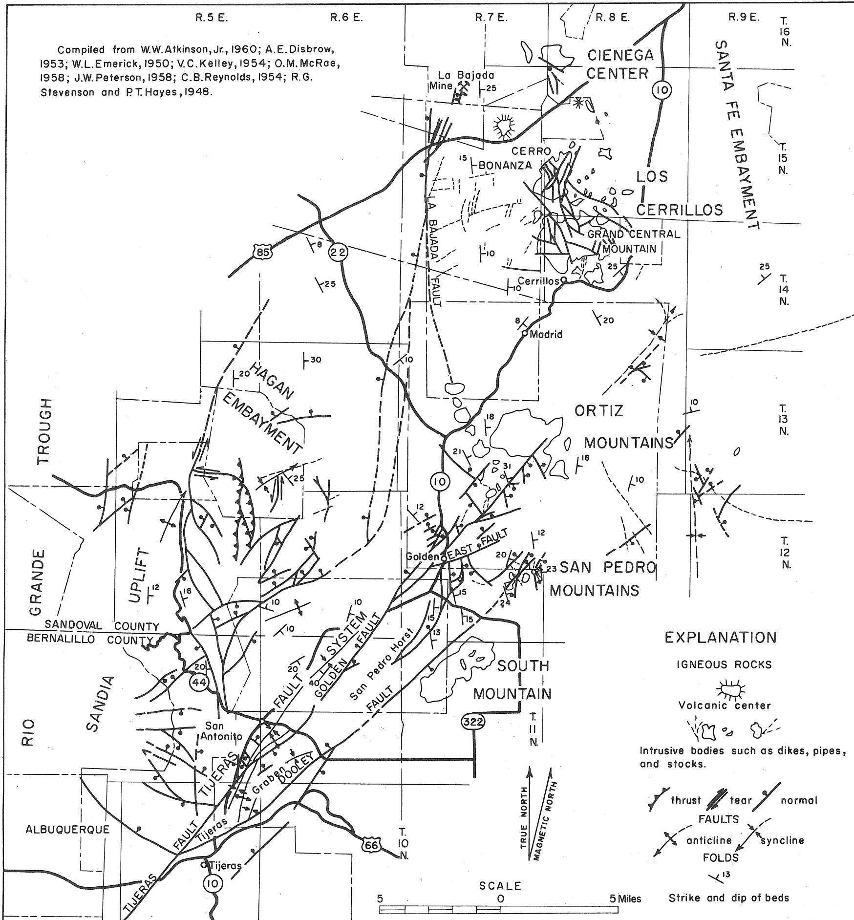
TECTONIC MAP OF THE SAN PEDRO-ORTIZ PORPHYRY BELT
