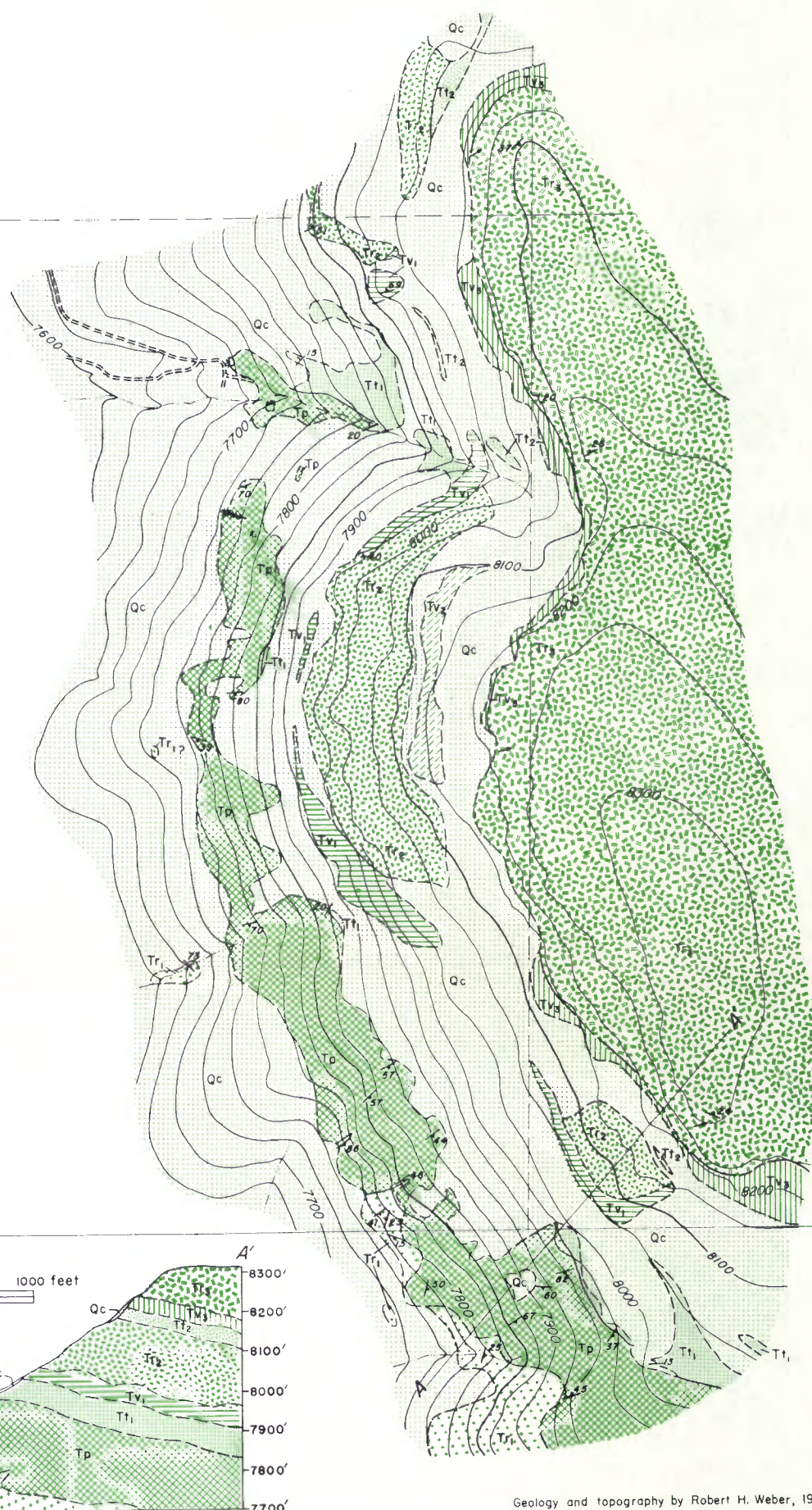
GEOLOGIC MAP OF THE STENDEL PERLITE DEPOSIT, SOCORRO COUNTY, NEW MEXICO
