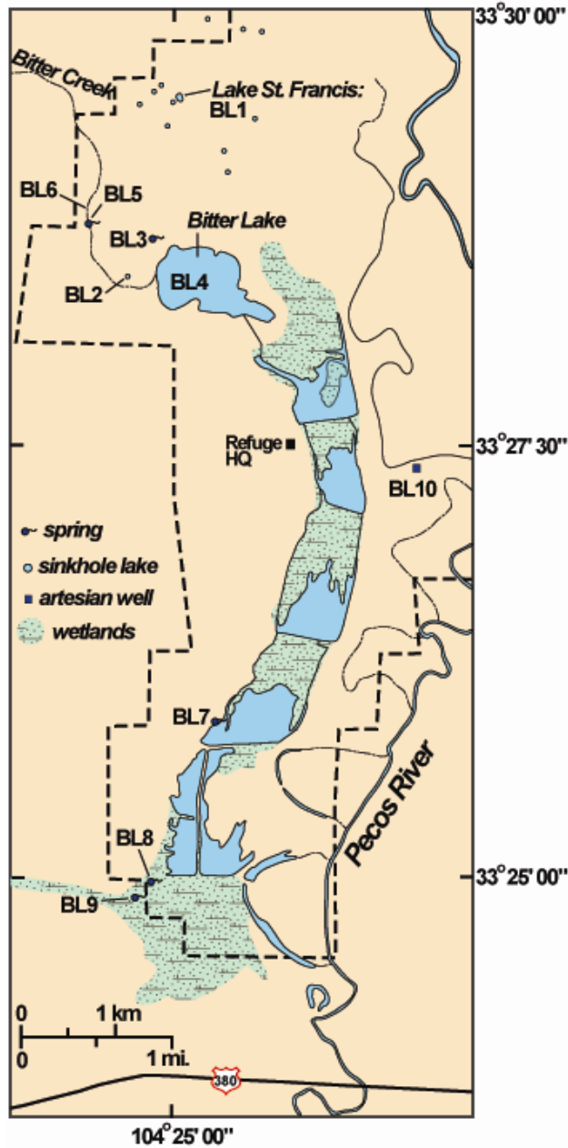
Figure 3: Detailed map of Bitter Lake National Wildlife Refuge, showing sample locations. Refuge boundary is indicated by dashed line.
