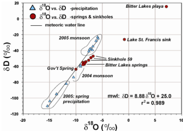
Figure 8: Stable isotopic composition of water samples collected from springs and sinkholes at Bitter Lake NWR relative to the meteoric water line for southeastern New Mexico.
