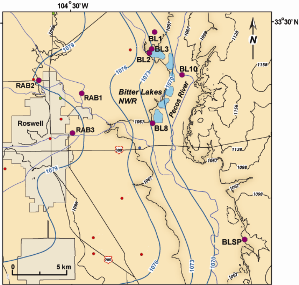
Figure 4: Map of central Chaves Co., NM, showing location of Bitter Lake National Wildlife Refuge (NWR). Heavy blue lines are contours of hydrostatic head (m) in the San Andres artesian aquifer. Light black lines are topographic contours (m). Note that elevation of hydrostatic head is above ground level in the vicinity of the Refuge. Small filled circles (red and green) are irrigation and monitoring wells completed in the artesian aquifer. Large filled circles (purple) are ^{14}\text{C} sampling stations.
