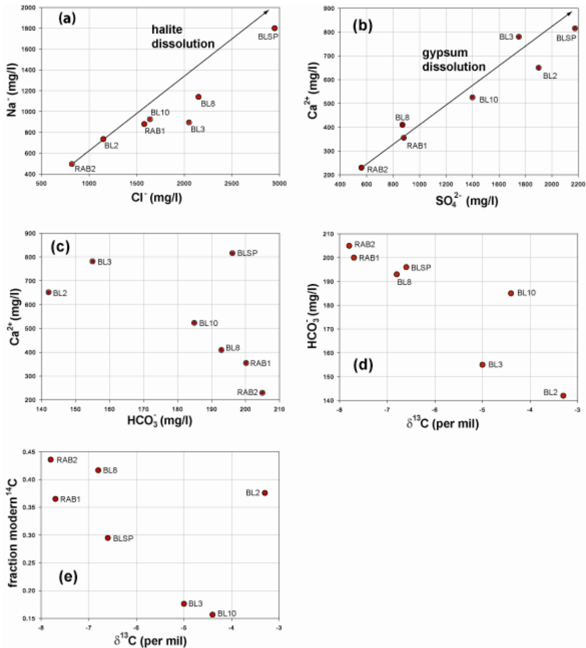
Figure 6: Hydrochemical data from Bitter Lake springs and artesian wells.
