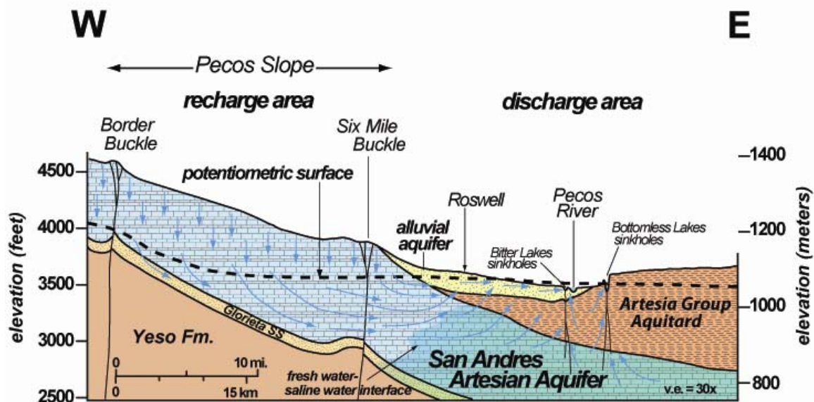
Figure 2: West-east hydrostratigraphic cross-section of the Roswell Artesian Basin, showing generalized direction of groundwater flow paths through the artesian aquifer system. Elevation is relative to sea level. Vertical exaggeration (v.e.) = 30X. Location of section shown in figure 1.
