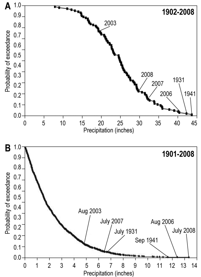
Figure 15 —Probability of exceedance curves for annual precipitation and monthly precipitation in Cloudcroft.
