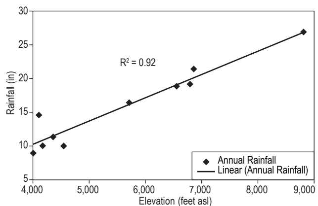
Figure 14 —Average annual precipitation versus elevation. The total annual precipitation at weather stations listed in Table 2 increases linearly with elevation, indicating that there is more precipitation at higher elevations than at lower elevations.
