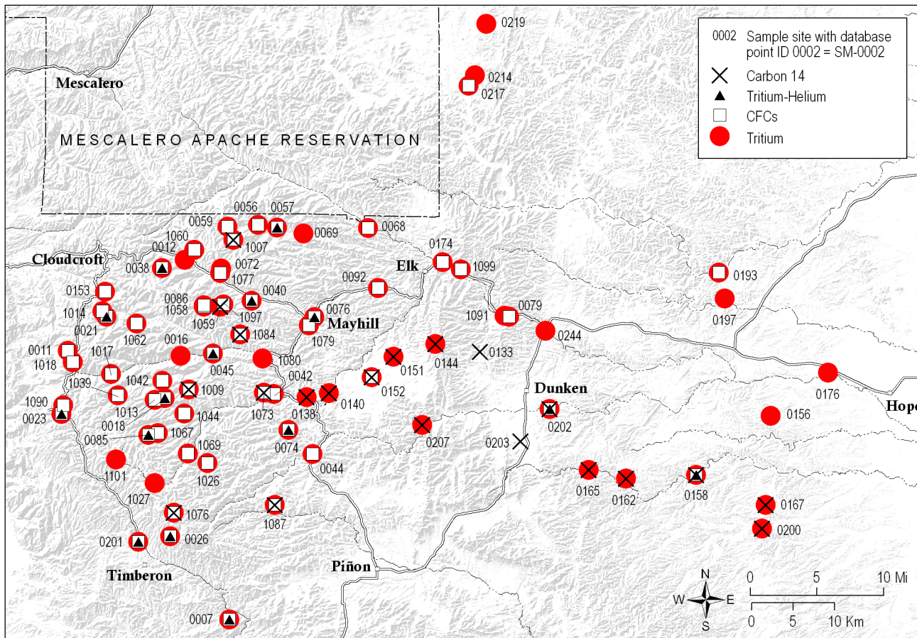
Figure 44 —Map showing sample locations for age-dating analyses. Environmental tracers used for age-dating include CFCs, tritium ( ^3\text{H} ), tritium-helium ( ^3\text{H}:^3\text{He} ), and carbon-14.
