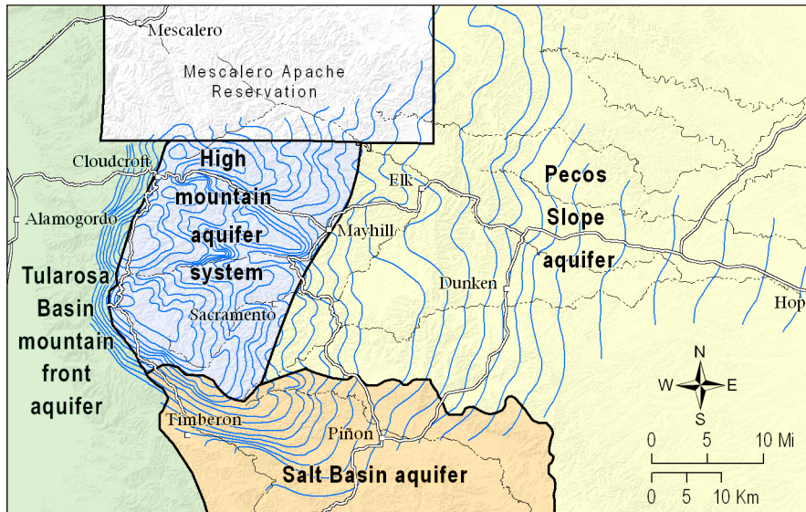
Figure 24 —Map of regional aquifer systems in the Sacramento Mountains. Blue lines are water-level elevation contours shown in Figure 18.
