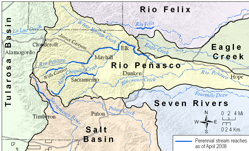
Figure 16 —Surface water drainage basins and perennial stream reaches. Few streams in the Sacramento Mountains are perennial. Perennial flow, depicted in dark blue, typically only occurs over short distances before infiltrating to shallow ground-water.
