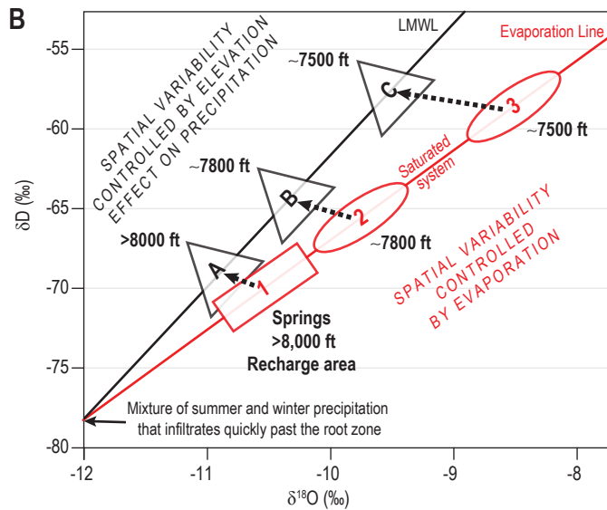
Figure 43 —Stable isotope signatures for different recharge mechanisms. A —Schematic diagram of identifying water stored in vadose zone (triangles), and water moving through saturated carbonate aquifer system (ovals). Symbols within triangles or ovals indicate process that control the isotopic composition of that water reservoir at that elevation. Black arrows show possible flow paths that include horizontal flow parallel to bedding planes in limestone and dolomite layers, and vertical leakage through intermediate vadose zone to a lower carbonate aquifer. Most water in saturated carbonate system originates from infiltration of precipitation at high elevations (>8,200 feet) that mixes in the subsurface. Movement of vadose zone water at lower elevations into the saturated system occurs due to large precipitation events such as those observed during the 2006 and 2008 monsoon seasons. B —Isotopic compositions of groundwater in carbonate aquifer system (evolves along evaporation line) and water stored in vadose zone (plots along LMWL). The flushing of vadose zone water into saturated system due to 2006 and 2008 monsoon seasons, caused isotopic composition of groundwater to shift towards vadose zone values.
