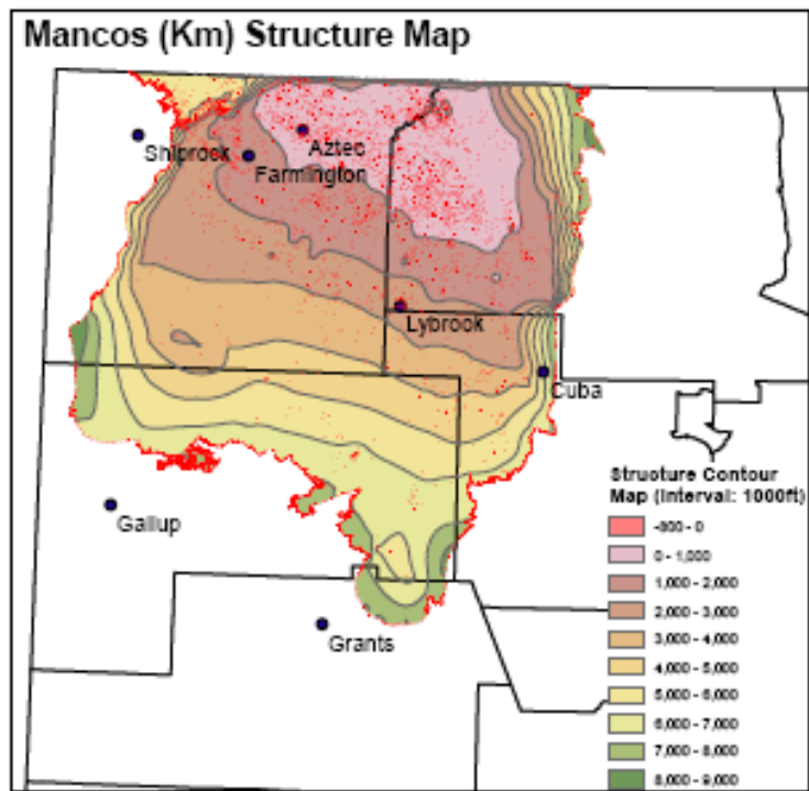
Figure 5. Top of Mancos structure contour map
