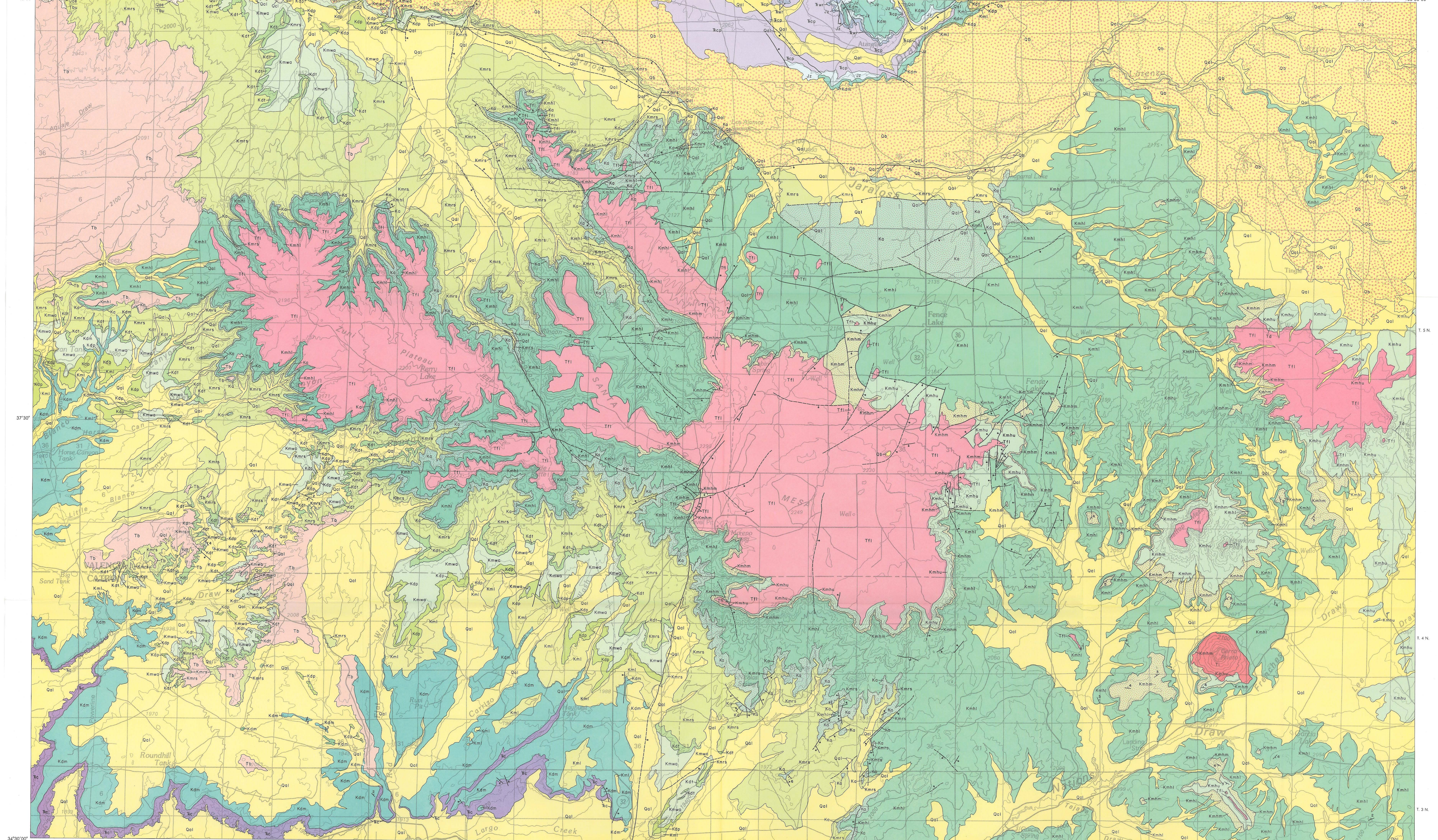
Geology and coal resources of Fence Lake 1:50,000 quadrangle, New Mexico (SW quadrant of Fence Lake 1:100,000 sheet)
