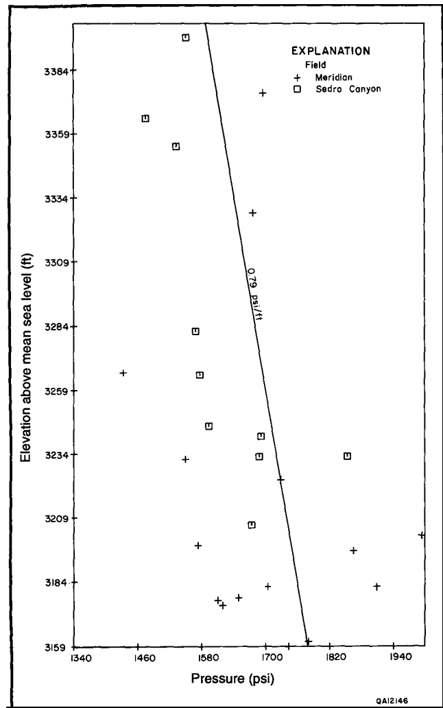
FIGURE 8.3—Fruitland Formation pressure-elevation plot, Sedro Canyon—Meridian 400 area (from Kaiser and Swartz, 1990). See Fig. 8.1 for area location. Vertical pressure gradient ( \sim 0.79 psi/ft) is the slope of the trend line and is much greater than hydrostatic gradient (0.433 psi/ft), which indicates strong potential for upward flow. Large vertical pressure gradient indicates reservoir heterogeneity and low vertical permeability. Large lateral pressure gradient (note wide pressure range at 3,184 ft [970 m]) also indicates reservoir heterogeneity.
