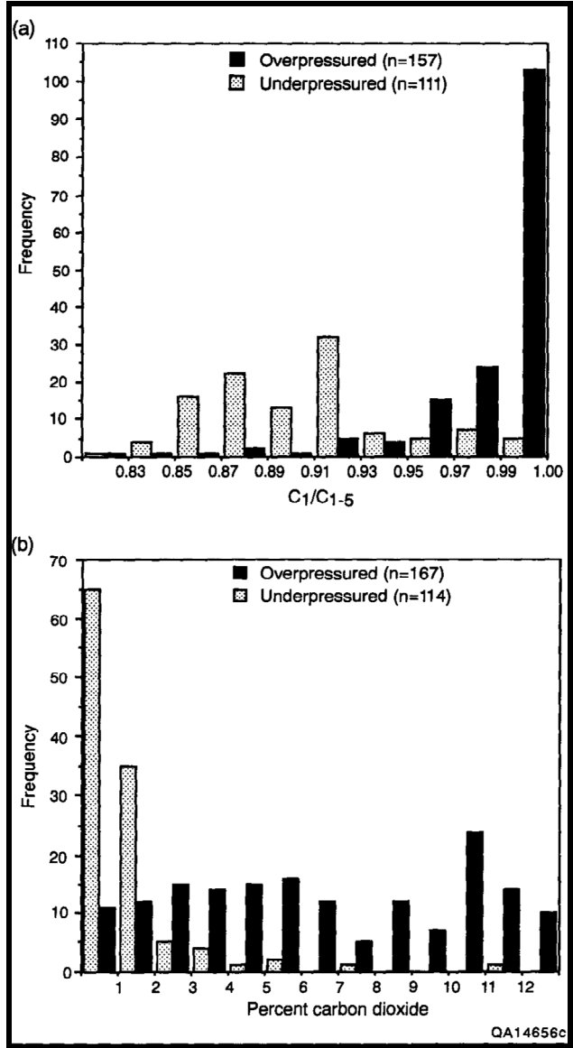
FIGURE 9.12—Histograms of (a) C 1 /C 1-5 values and (b) carbon dioxide content of gases from overpressured and underpressured Fruitland coal beds. Gases from the overpressured, thermally more mature coal in the northern basin are significantly drier than coalbed gases from the underpressured area. Gases from underpressured coal beds generally contain less than 2% carbon dioxide, whereas gases from overpressured coal beds commonly contain more than 2% carbon dioxide. The bimodal distribution of carbon dioxide in the overpressured gases primarily reflects the high carbon dioxide content in samples from the Meridian 400 area.
