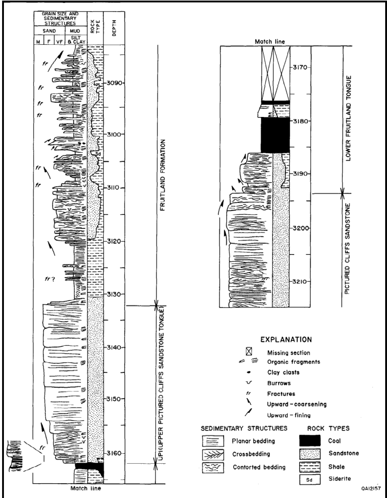
FIGURE 4.6—Core description of Pictured Cliffs Sandstone, lower Fruitland tongue, upper Pictured Cliffs tongue (UP1), and Fruitland Formation in Blackwood and Nichols NEBU No. 403 (see Fig. 4.5).
