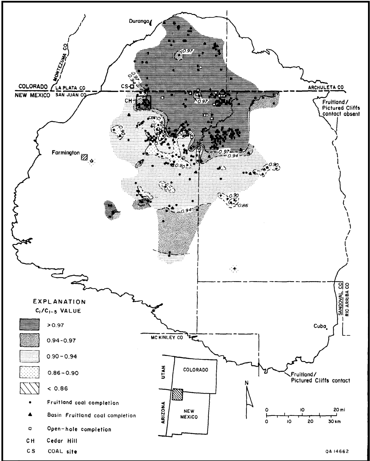
FIGURE 9.9— C_1/C_{1.5} values of Fruitland coalbed gases. Gases derived from higher rank coals (vitrinite reflectance values >0.8\% ) in the overpressured area generally have C_1/C_{1.5} values greater than 0.97. Isotopic data and the abrupt transition from very dry to wet gases suggest that dry gases in the northern basin are derived from both thermogenic and biogenic sources.
