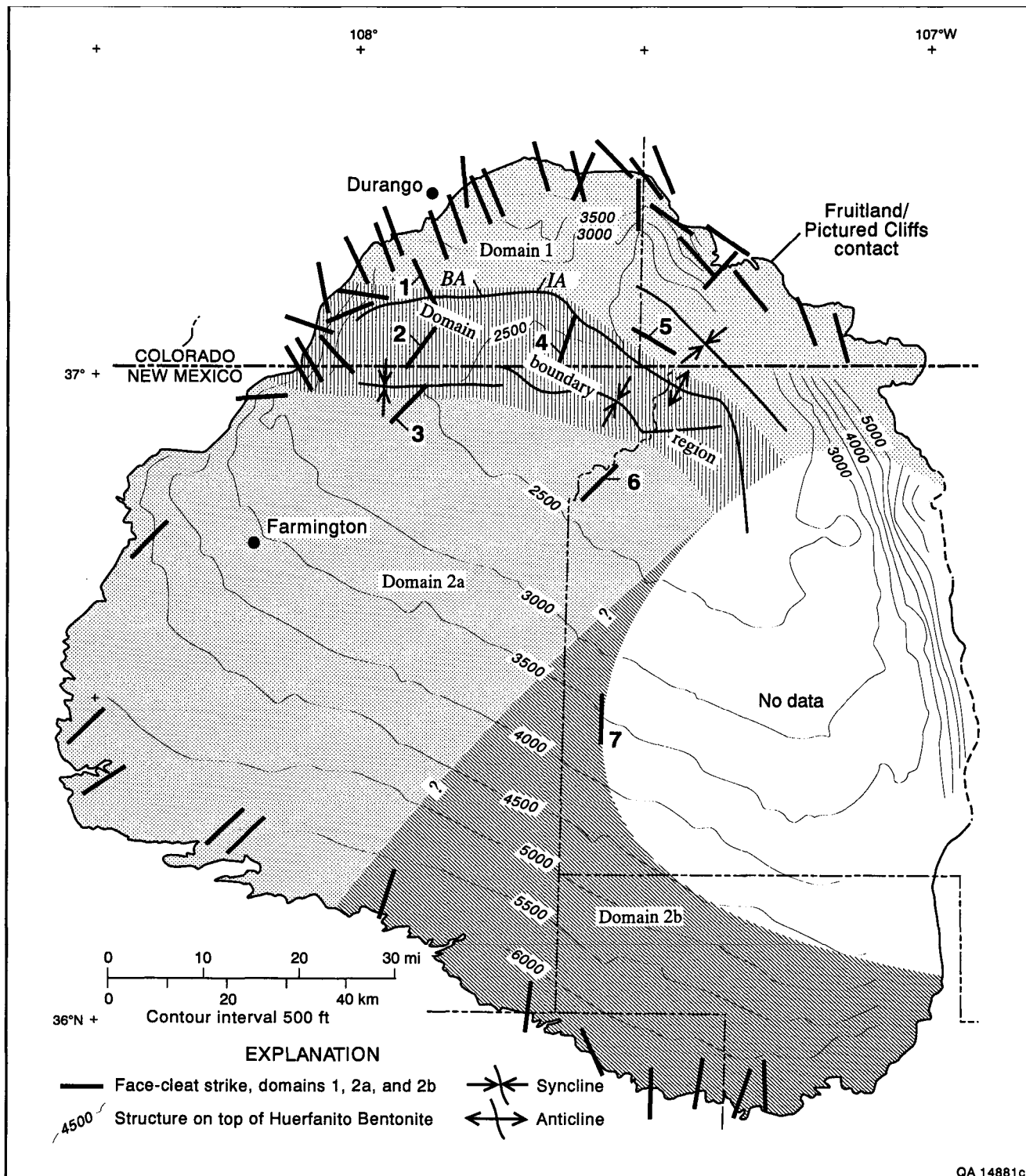
FIGURE 5.12—Structure map of San Juan Basin, contoured on the Huerfanito Bentonite, and face-cleat strikes and face-cleat-strike domains of the Fruitland Formation coal seams in the San Juan Basin. Domain boundaries are gradational and approximately located. Boldface numbers indicate wells with oriented core used in this study (see Table 5.3). Locations of stations are indicated in Table 5.1. BA–IA = Bondad–Ignacio anticline.
