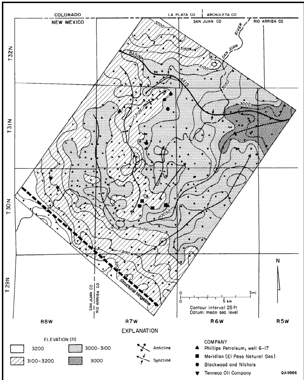
FIGURE 4.3—Elevation of the top of the Pictured Cliffs Sandstone results primarily from structural features (compare with Fig. 4.2) and secondarily from sedimentary fades changes.
