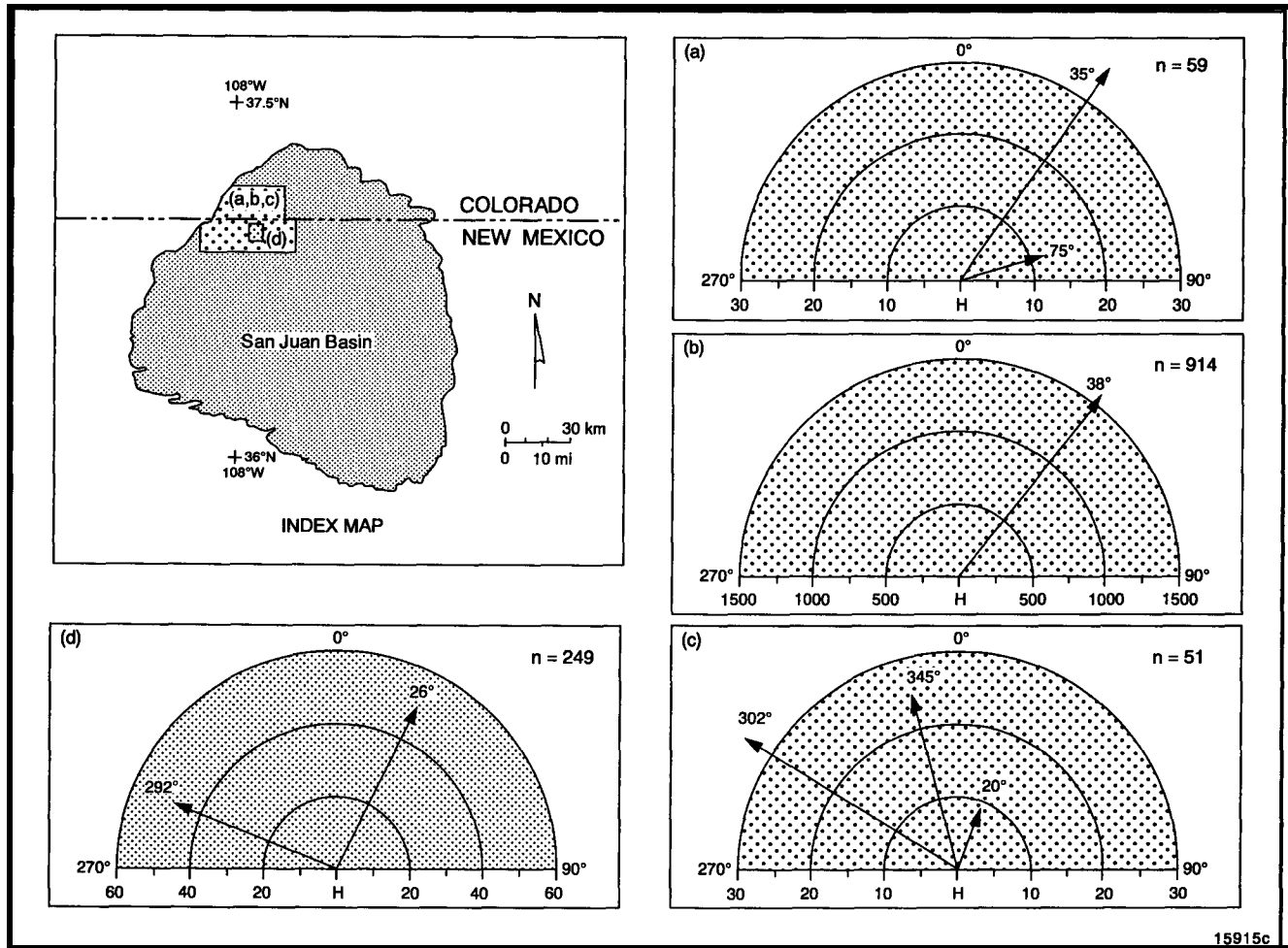
FIGURE 7.5—Polar graphs of Bernshtein accuracy criterion ( H ) for lineaments in this and three previous studies. Only vector sums of lineament azimuths that are significant at the p = 0.01 level are shown. See inset for area covered by each study. Stipple patterns represent areas that correspond to like data on graphs. Note that a, b, and c lineaments are from different studies in the northwestern San Juan Basin. (a) Landsat lineaments, this study. (b) Aerial photolineaments, Kelley and Clinton (1960). (c) Landsat lineaments, Knepper (1982). (d) Aerial photolineaments in Cedar Hill field area, Decker and others (1989). Landsat lineaments mapped by Decker and others (1989) are insufficient ( n = 11 ) to produce a meaningful value for H .
