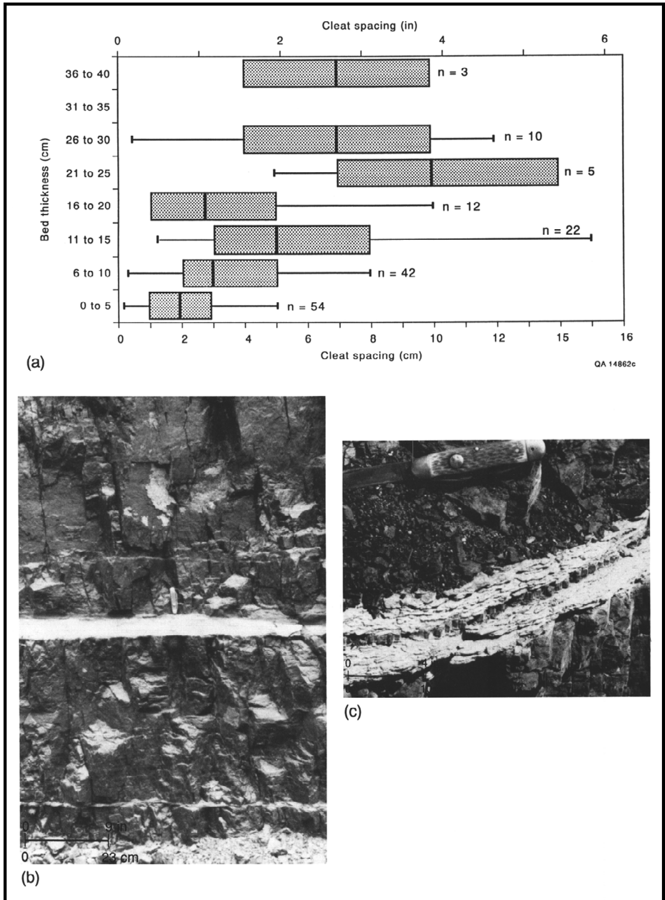
FIGURE 5.8—Illustrations of cleat spacing patterns. (a) Cleat spacing grouped by equal bed-thickness intervals. Center half of data is represented by a rectangle (box) and median is indicated by a bar. (b) Widely spaced primary cleats in thick coal bed, Navajo mine. (c) Close cleat spacing in thin coal bed, Navajo mine.
