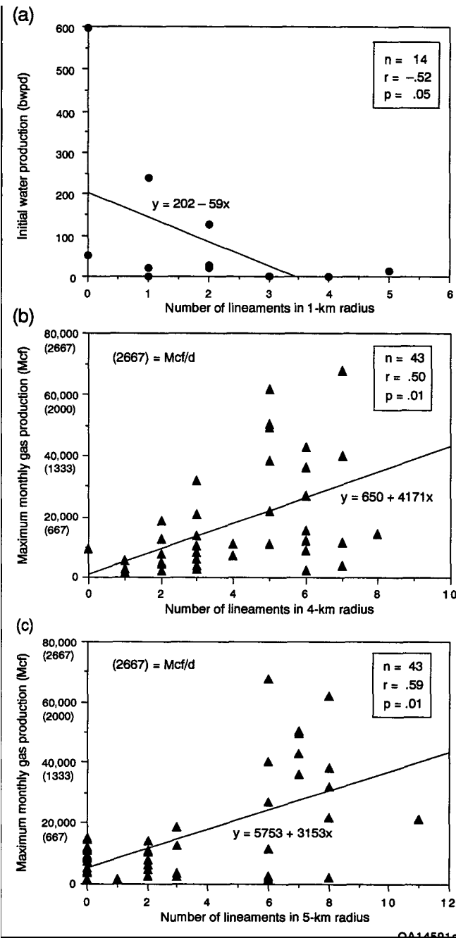
FIGURE 7.14—Graphs of production data versus number of Landsat lineaments within a given radius of a well. (a) IPW versus lineaments in a 0.6-mi (1-km) radius (Decker and others, 1989). Negative correlation coefficient indicates that as number of lineaments near a well increases, IPW decreases, the reverse of the expected result. (b) MMG versus Landsat lineaments in a 2.5-mi (4-km) radius (this study). (c) MMG versus Landsat lineaments in a 3.1-mi (5-km) radius (Knepper, 1982). Positive correlations for (b) and (c) indicate that production increases as the number of lineaments increases, as expected. Applicability of these correlations to exploration is questionable, given the size of the radii around the wells.
