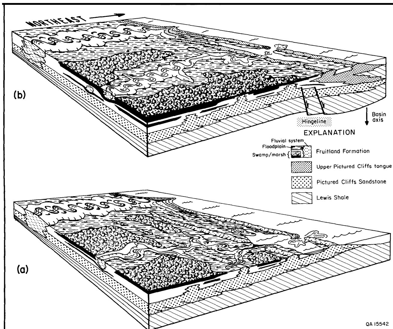
FIGURE 2.20—Depositional model of Fruitland coal seams in the Navajo Lake area. (a) Peat is deposited behind, and overrides, abandoned and foundering Pictured Cliffs shoreline sandstones that occur inland and downdrift of a postulated wave-dominated delta. Area is crossed only by minor fluvial feeders that shift periodically. (b) Intermittent subsidence along basin axis temporarily halts regression, causing a shoreline stillstand and allowing accumulation of thick, extensive peat deposits. Not to scale. From Ayers and Zellers, 1988.
