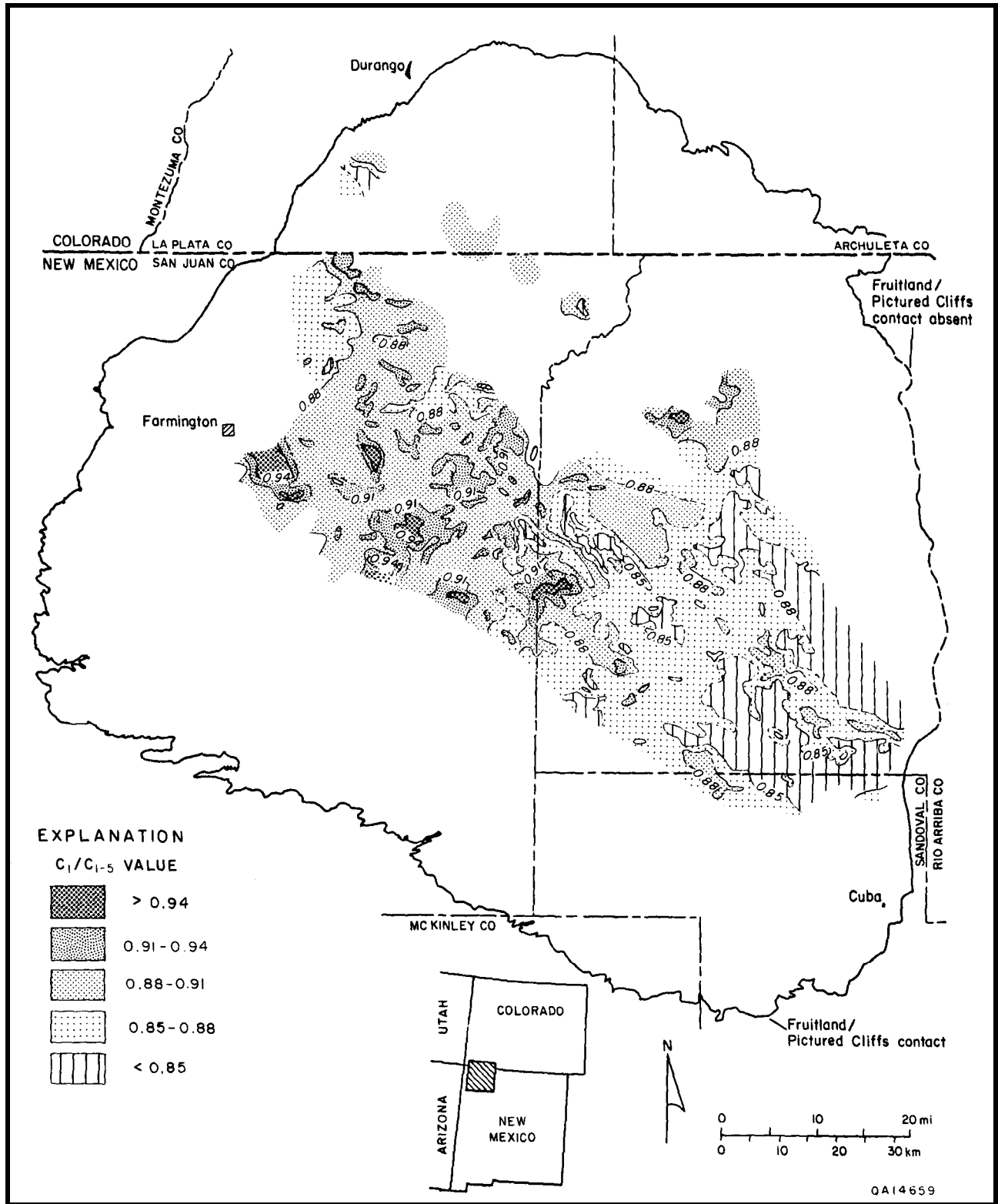
FIGURE 9.16—C 1 /C 1-5 values of Pictured Cliffs sandstone gases. Pictured Cliffs gases in the southeastern part of the trend are chemically wetter than gases produced from the northwestern part of the trend. The northeast-trending area of drier gases (C 1 /C 1-5 values >0.91) in east-central San Juan County coincides with areas where thicker Fruitland coal beds overlie the sandstones, suggesting that coalbed gases may have migrated downward. Gas analyses from more than 5,500 wells were used to construct this map.
