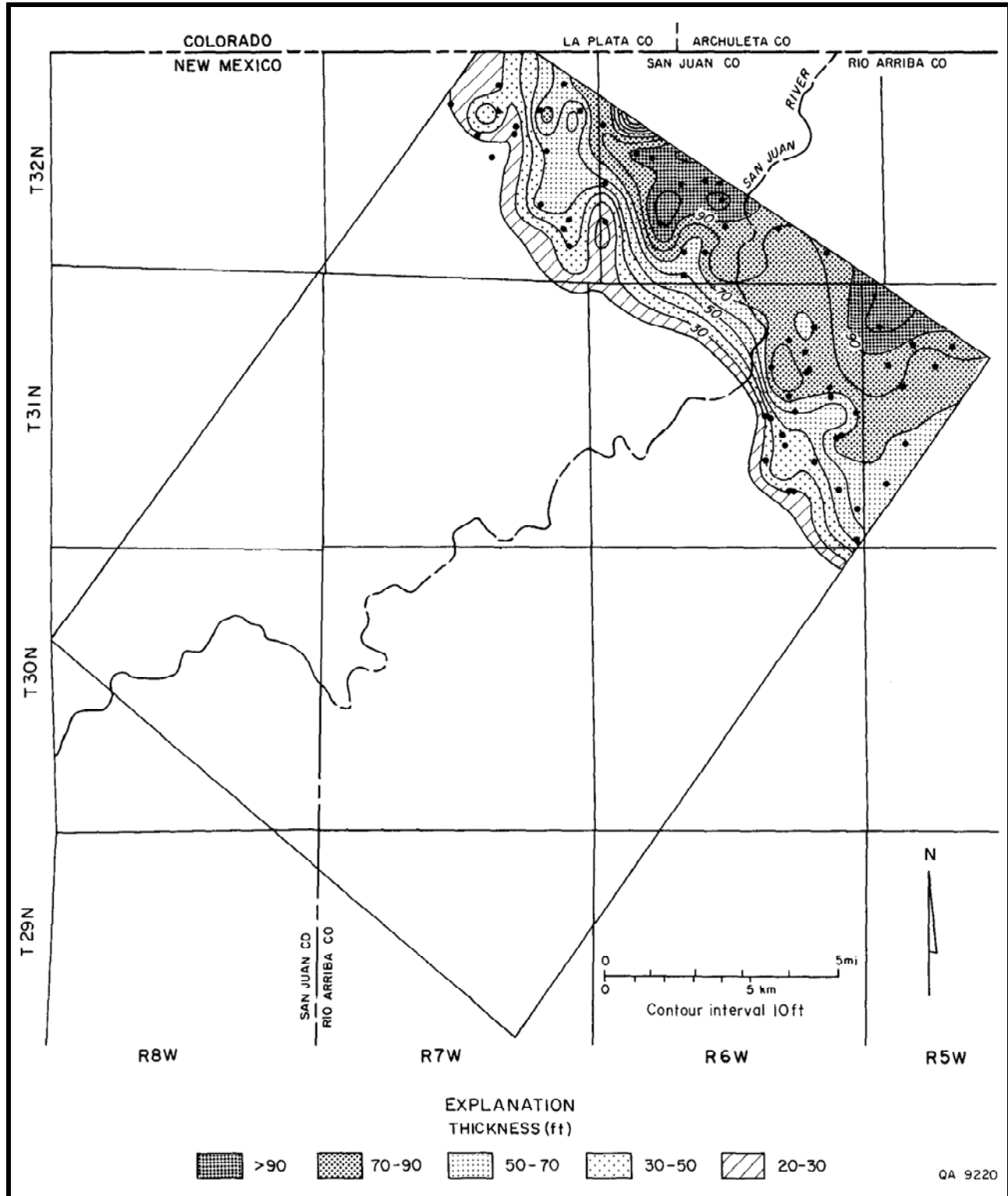
FIGURE 4.9—Sandstone isolith map of UP2 (Fig. 4.1). Depocenter of strike-elongate coastal sandstone is offset basinward of UP1 (Fig. 4.8). Area mapped is where net sandstone thickness exceeds 20 ft (6 m).
