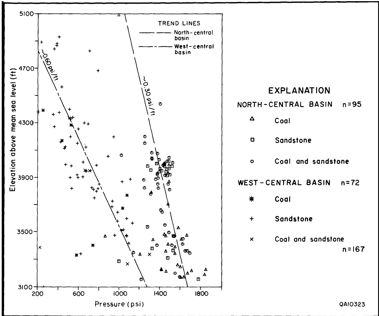
FIGURE 8.5—Fruitland Formation pressure-elevation plot, San Juan Basin (modified from Kaiser and Swartz, 1990). Vertical pressure gradient ( \sim 0.30 and \sim 0.60 psi/ft) is the slope of the respective trend line. Ground-water flow is potentially downward in the north-central part of the basin (vertical gradient < hydrostatic gradient, 0.433 psi/ft) and upward in the west-central part of the basin (vertical gradient > hydrostatic gradient). Coal and sandstone values lie along the same trend lines, indicating regional pressure communication between interbedded coal seams and sandstones.
