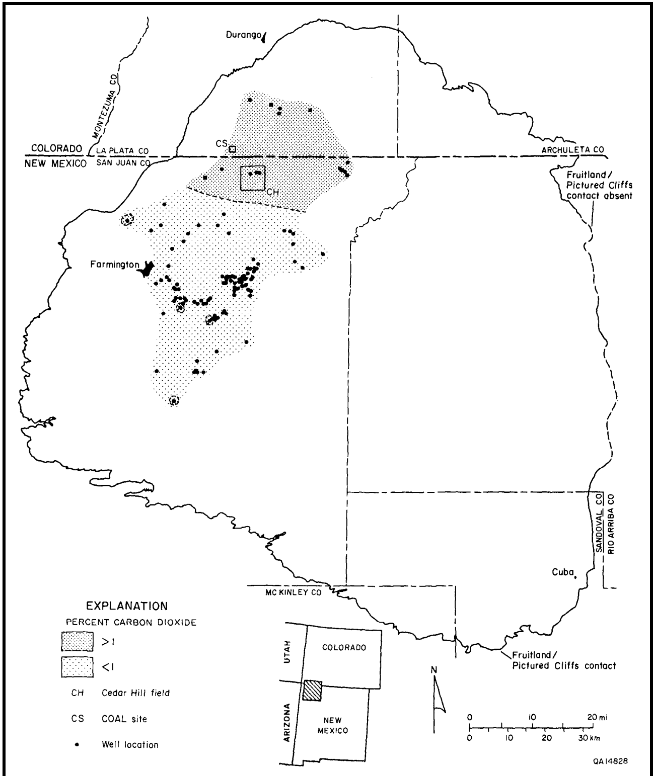
FIGURE 9.7—Carbon dioxide content of Fruitland sandstone gases. Fruitland sandstone gases in the northern basin contain slightly more carbon dioxide than do gases in the southern basin.
