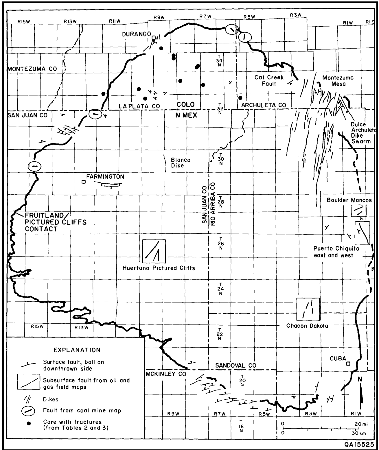
FIGURE 5.1—Faults and dikes in the San Juan Basin
