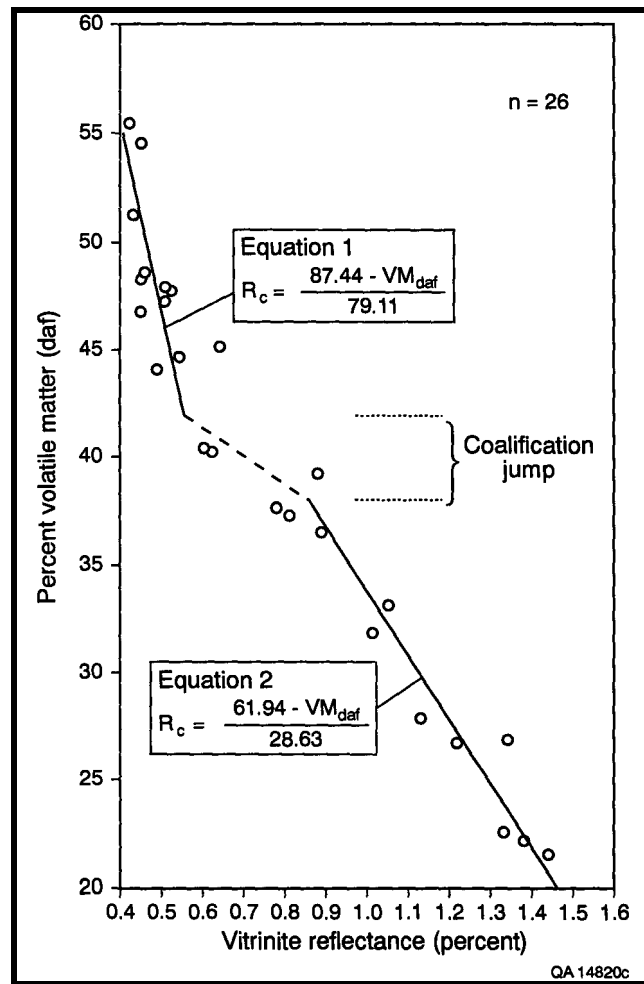
FIGURE 9.1—Relationship between vitrinite reflectance and volatile matter content of Fruitland coal. Two distinct linear trends are separated by an interval where vitrinite reflectance values increase abruptly with only a minor decrease in volatile matter (dry, ash-free basis). This coalification jump reflects the generation of bitumen from hydrogen-rich components of the coal.
