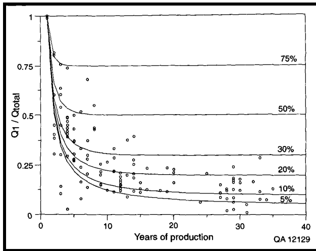
FIGURE 10.1—Q plot, Fruitland Formation sandstone wells.
