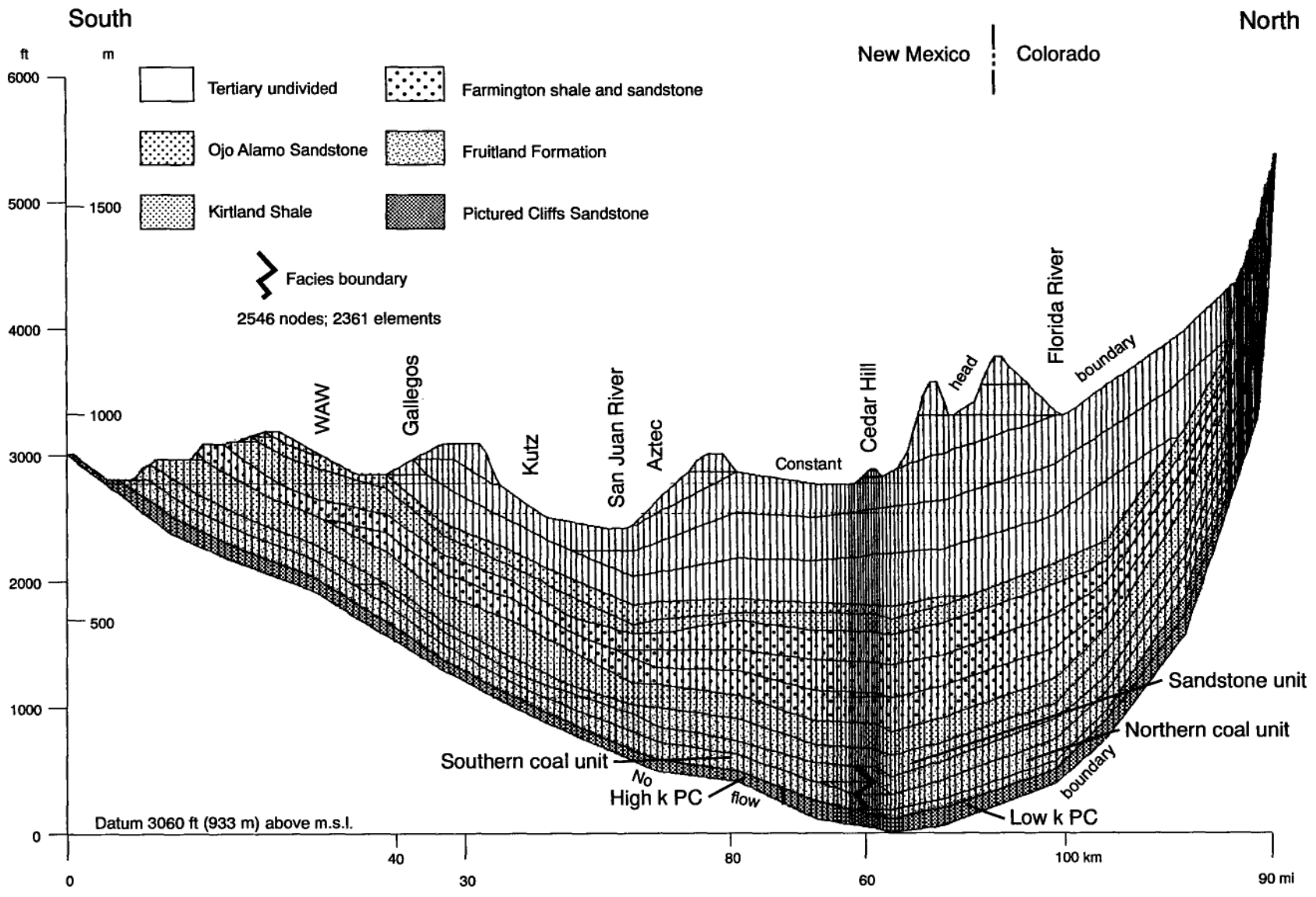
FIGURE 8.21—Finite-element mesh of major hydrogeologic units above the Lewis Shale, San Juan Basin. Units are assigned permeabilities that vary among simulations. The upper surface is a constant head boundary corresponding to the water table. The lower surface is a no-flow boundary corresponding to the contact between the Pictured Cliffs Sandstone and Lewis Shale. Vertical exaggeration 50x . See Fig. 8.1 for line of section.
