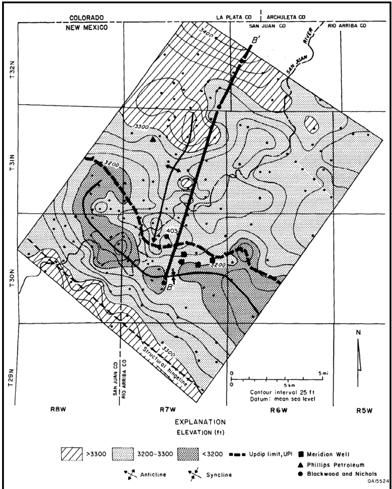
FIGURE 4.19—Structure map of upper Fruitland coal seam in Fig. 4.16. Attitude of the coal bed differs markedly from that of the Huerfanito Bentonite and the Pictured Cliffs Sandstone (Figs. 4.2 and 4.4, respectively). Structural trough occurs southwest of the pinch-out of UPI. Cross section B–B' is in Fig. 4.18.
