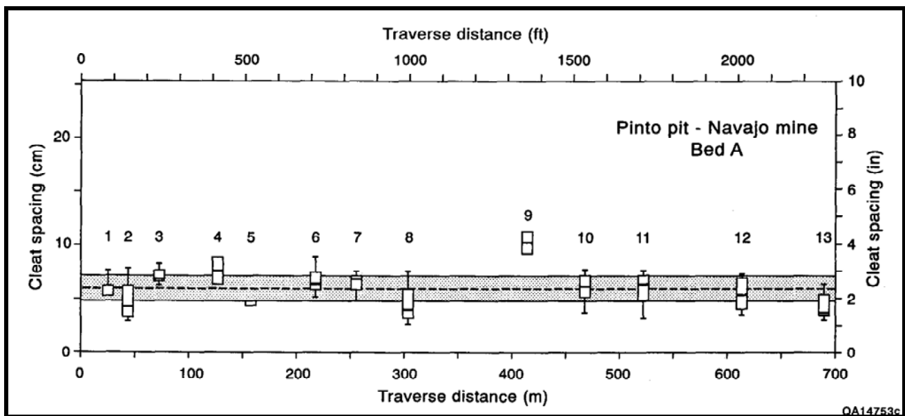
FIGURE 5.5—Cleat spacing versus traverse distance in a bed of uniform dip, thickness, and composition, Navajo mine. Center half of the data at each station is represented by a rectangle (box) and median is indicated by a bar. Dashed line and shaded area represent mean and one standard deviation of measurements from all stations.
