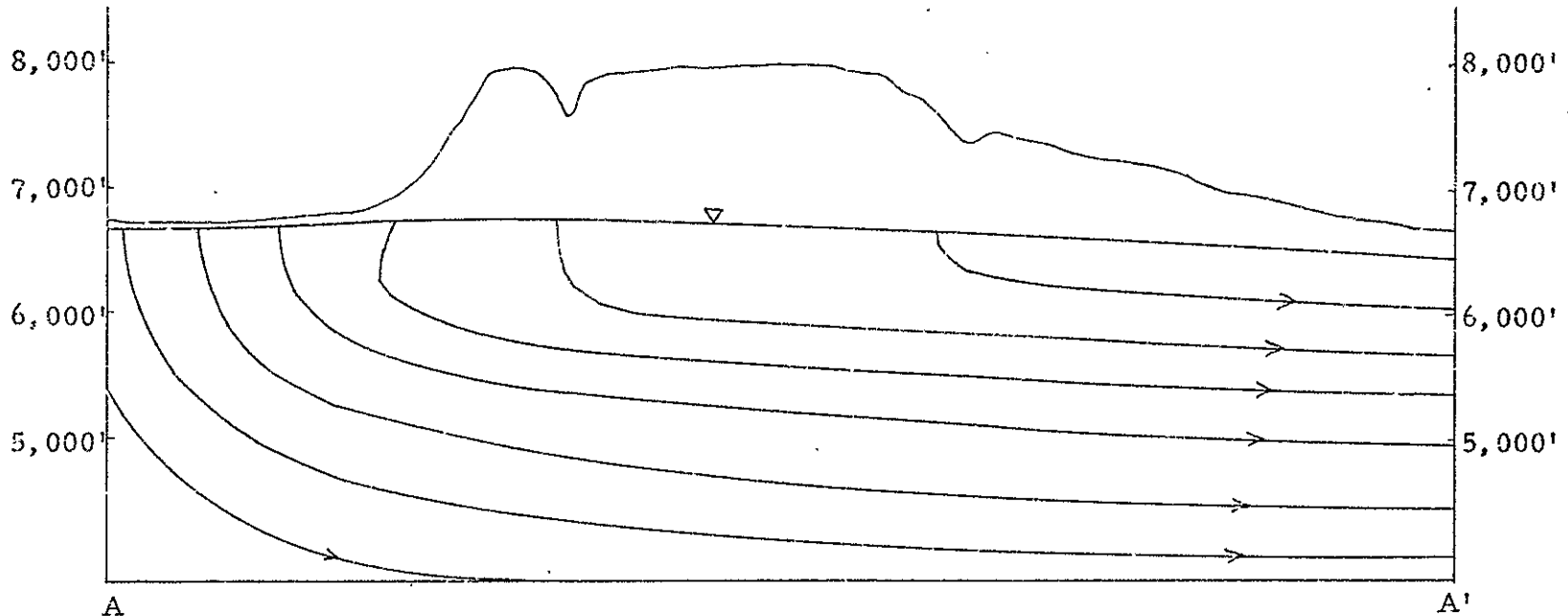
A North Fig. 2 Fig. 2 Idealized cross section with inferred groundwater flow paths (See Map 1 for location.) South A'
