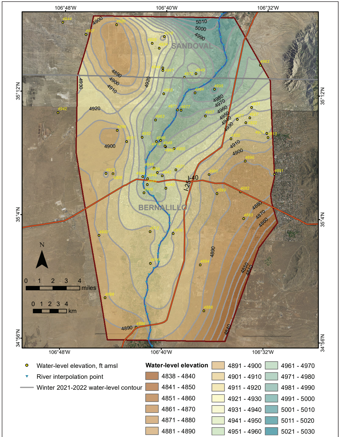
Figure 4. Winter 2021–2022 water-level elevation surface. Wells with measurements used in the geostatistical interpolation to create the surface are shown in yellow.
