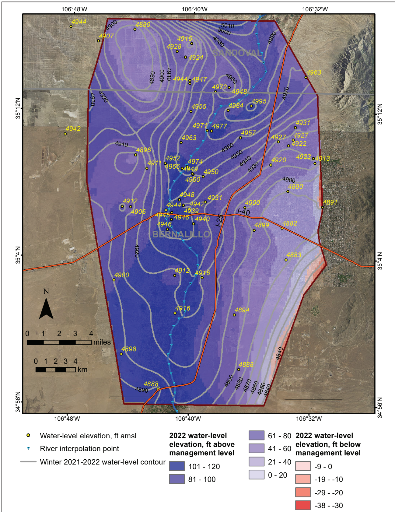
Figure 9. Winter 2021–2022 water-level surface with respect to the 110-ft drawdown management level. Water levels above the management level are in shades of blue and those below are in shades of red.
