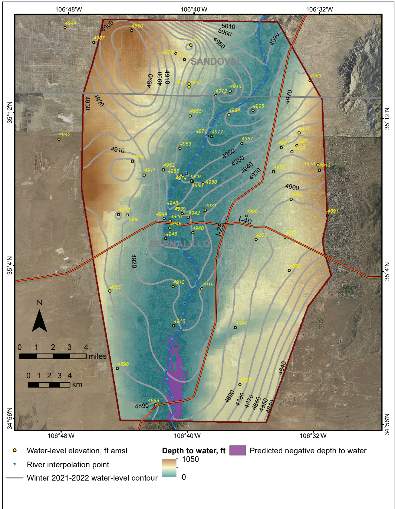
Figure 6. Depth to water based on the winter 2021–2022 water-level surface. Areas where the water level is predicted to be at or above the ground surface are shown in purple. See text for discussion.
