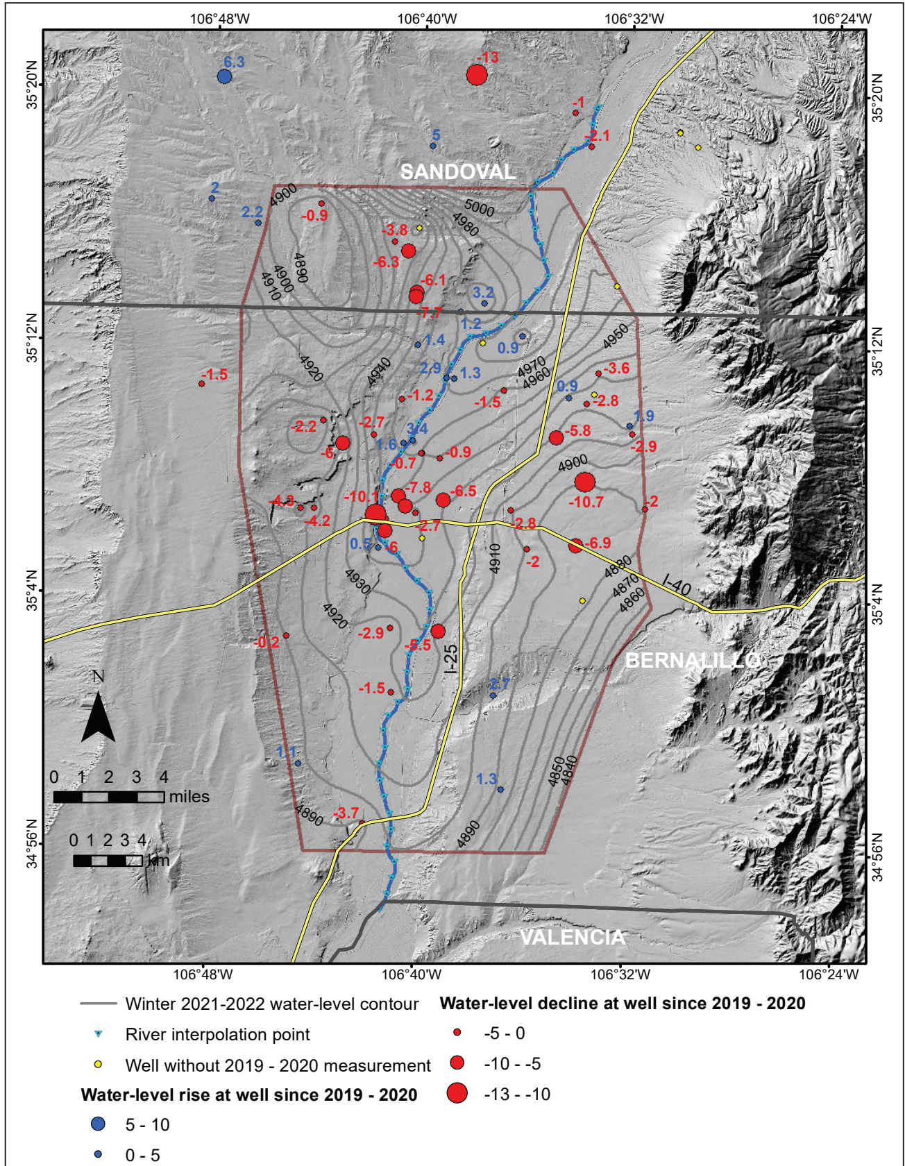
Figure 8. Change in water levels at wells from winter 2019–2020. Rises (positive) are in blue and declines (negative) are in red. Unlabeled yellow wells did not have measurements in winter 2019–2020.
