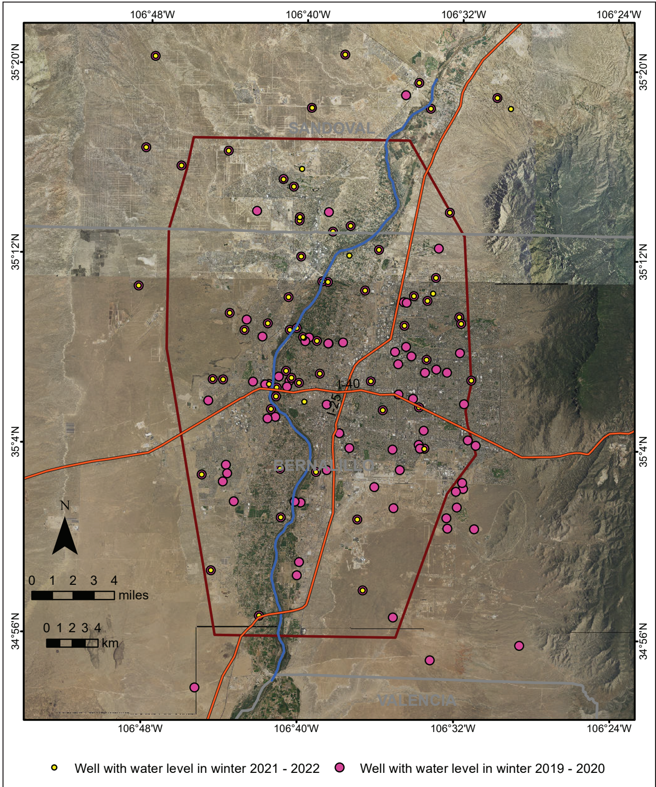
Figure 3. Map illustrating wells with water-level measurements in winter 2019–2020 and winter 2021–2022.
