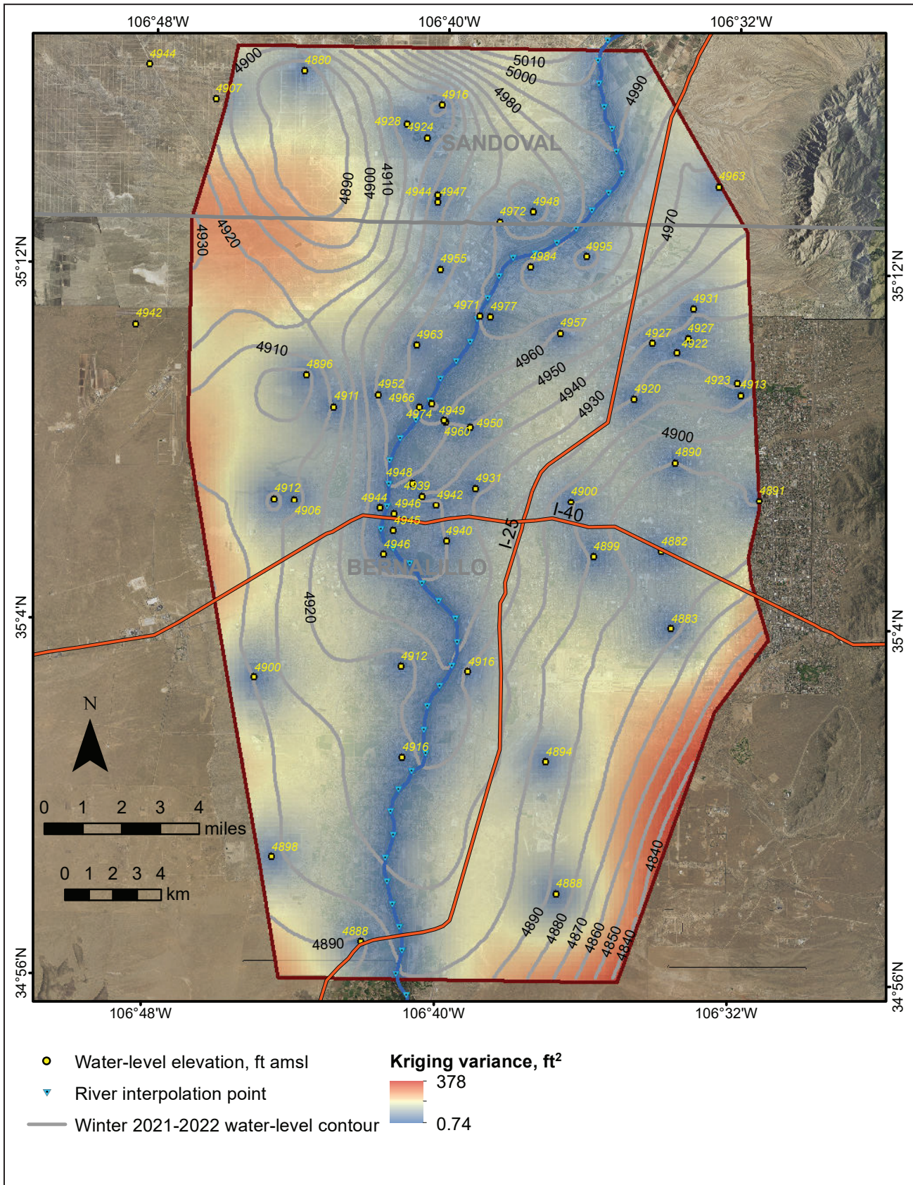
Figure 5. Kriging variance of the recent (2021–2022) water-level elevation surface. Lower variance corresponds to more-reliable results. Wells with measurements used in the geostatistical interpolation to create the surface are shown in yellow.
