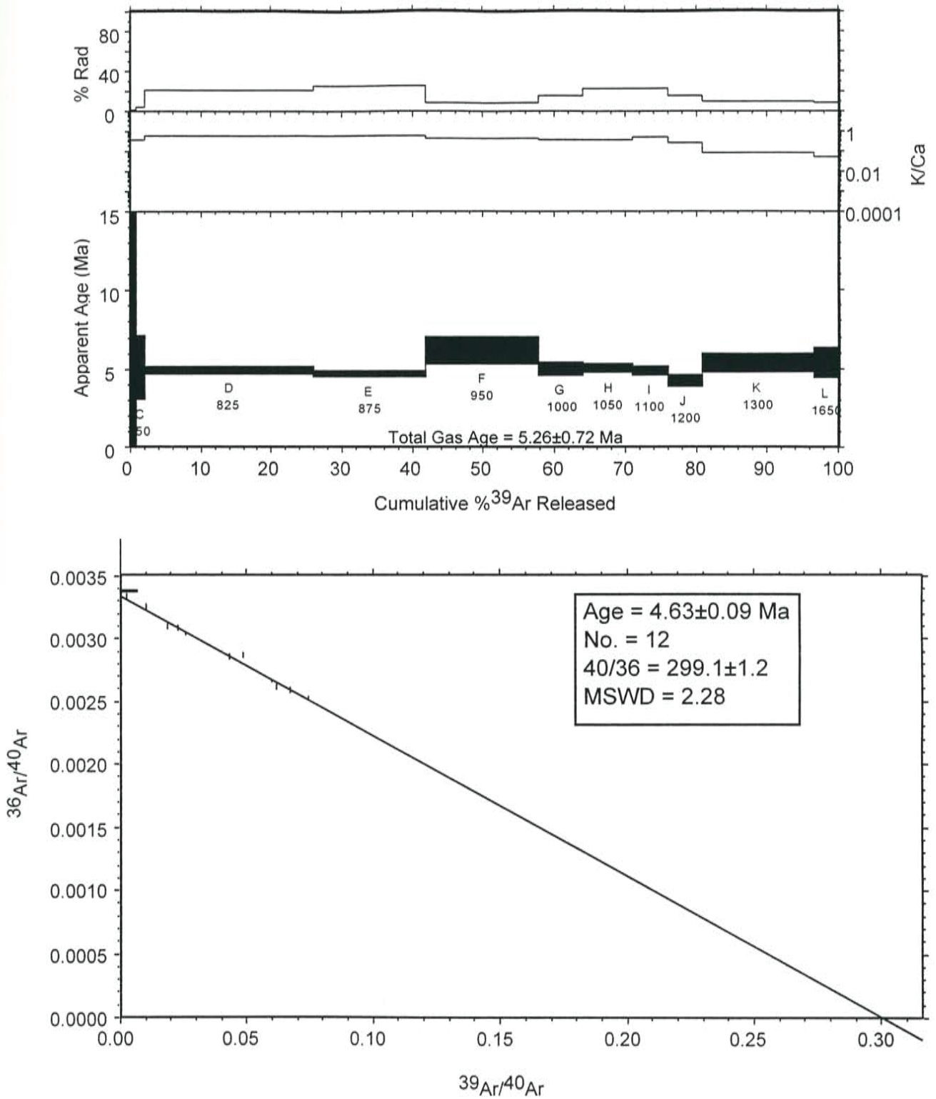
RA-080, Servilleta Basalt, Commanche Rim, groundmass concentrate
