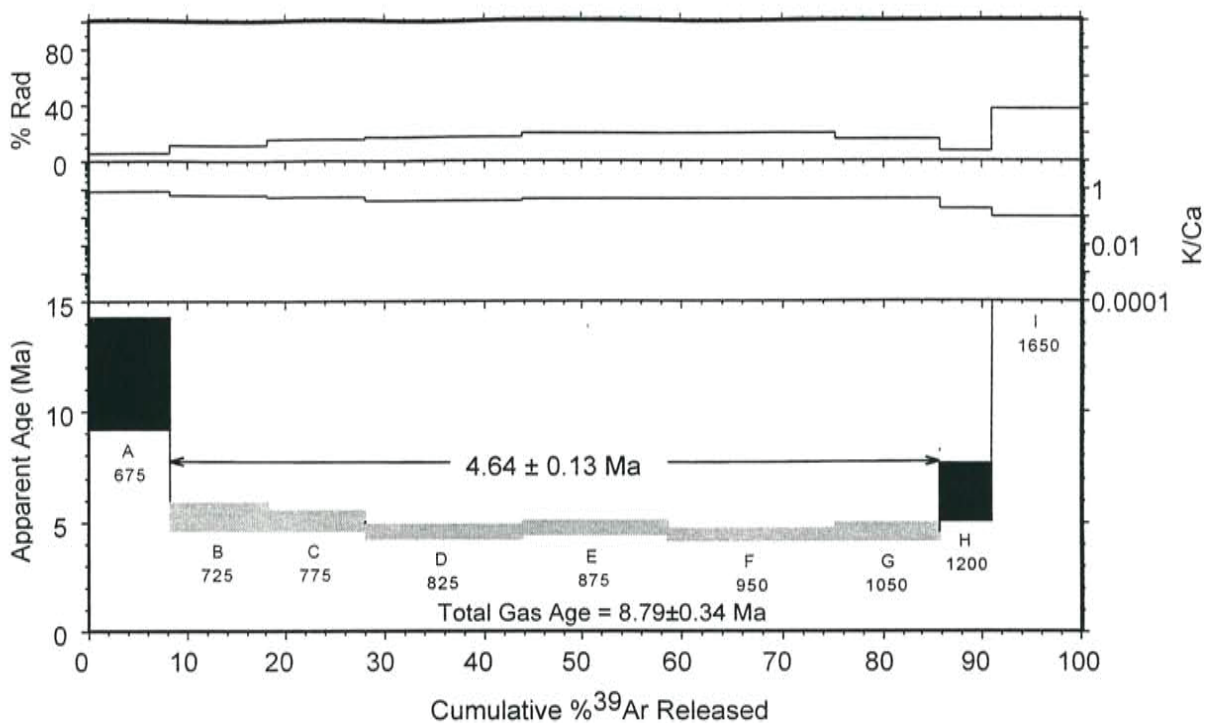
RA-056, basalt, Mesa Vibora, groundmass concentrate
