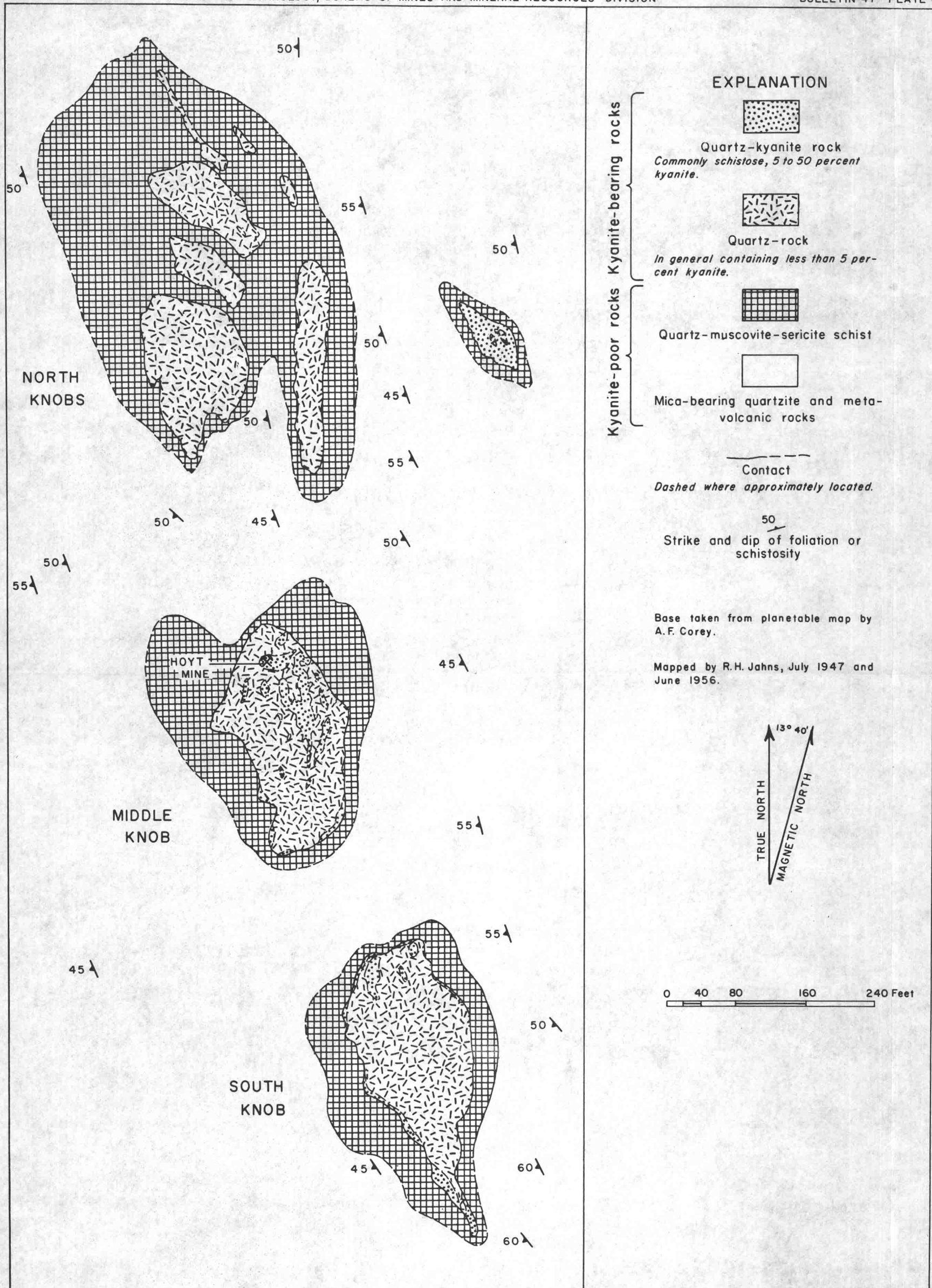
GEOLOGY OF THE BIG ROCK AREA
