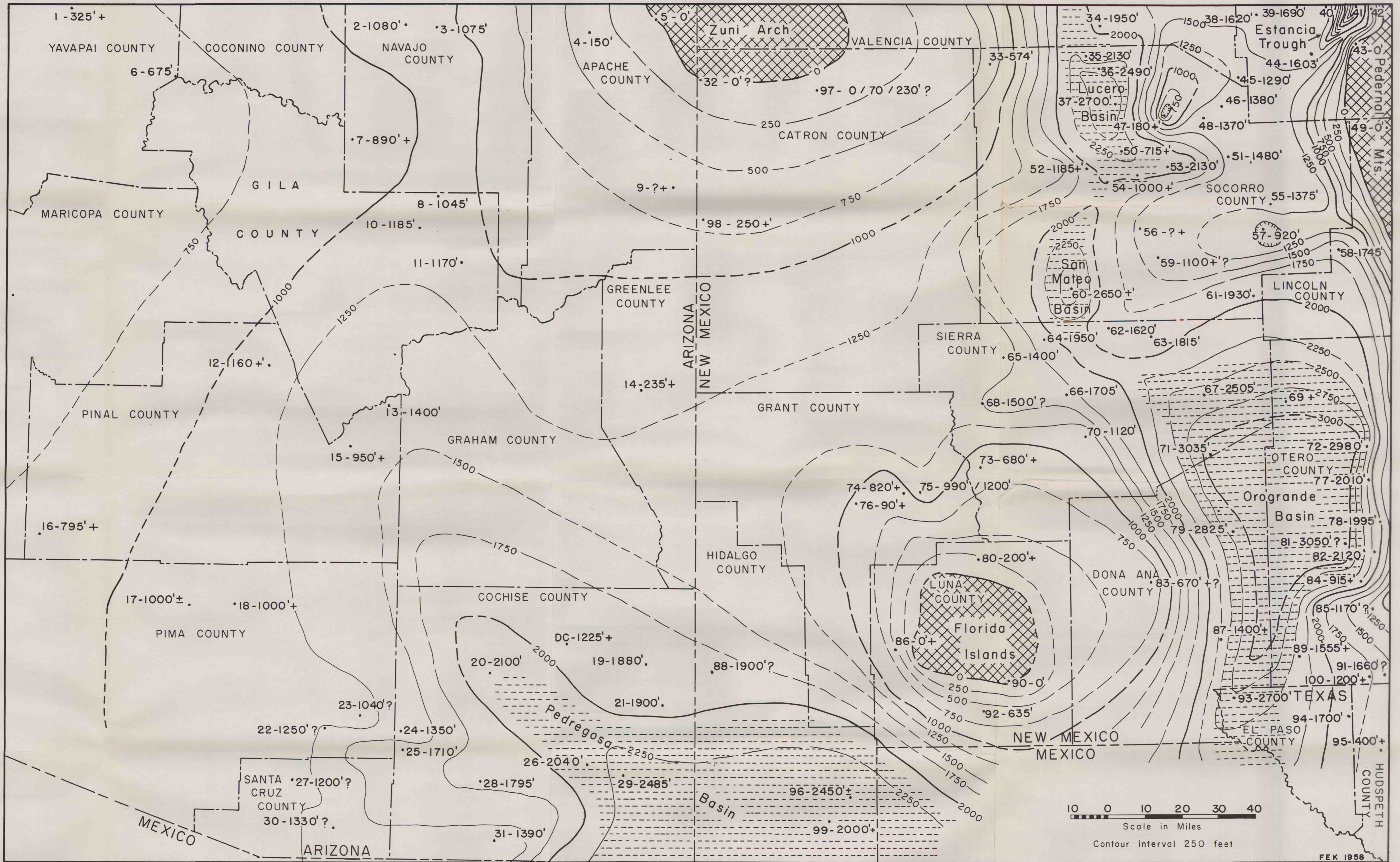
ISOPACH MAP FOR PENNSYLVANIAN OF SOUTHWESTERN NEW MEXICO AND SOUTHEASTERN ARIZONA AT END OF PENNSYLVANIAN PERIOD
