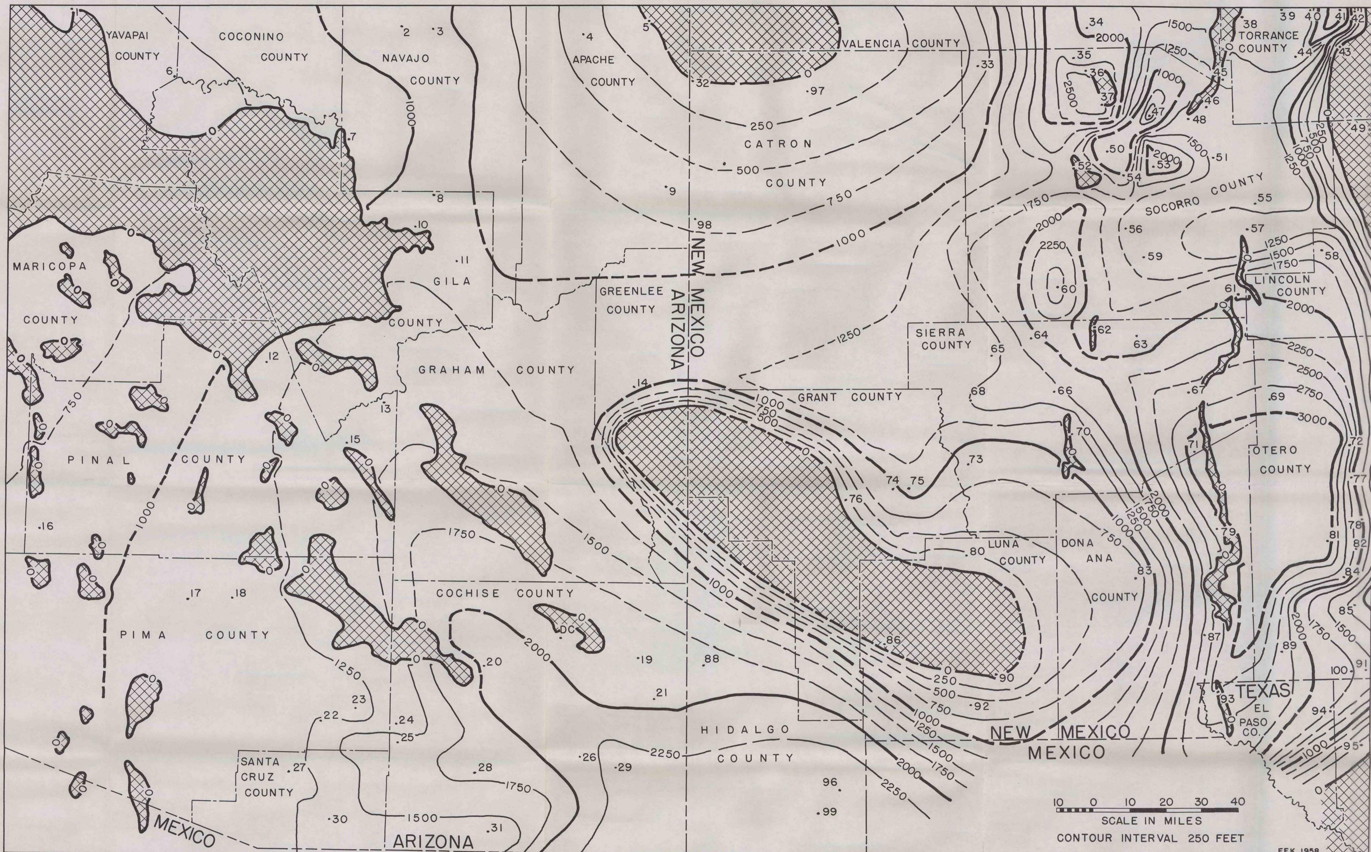
PRESENT ISOPACH MAP OF PENNSYLVANIAN ROCKS OF SOUTHWESTERN NEW MEXICO AND SOUTHEASTERN ARIZONA
