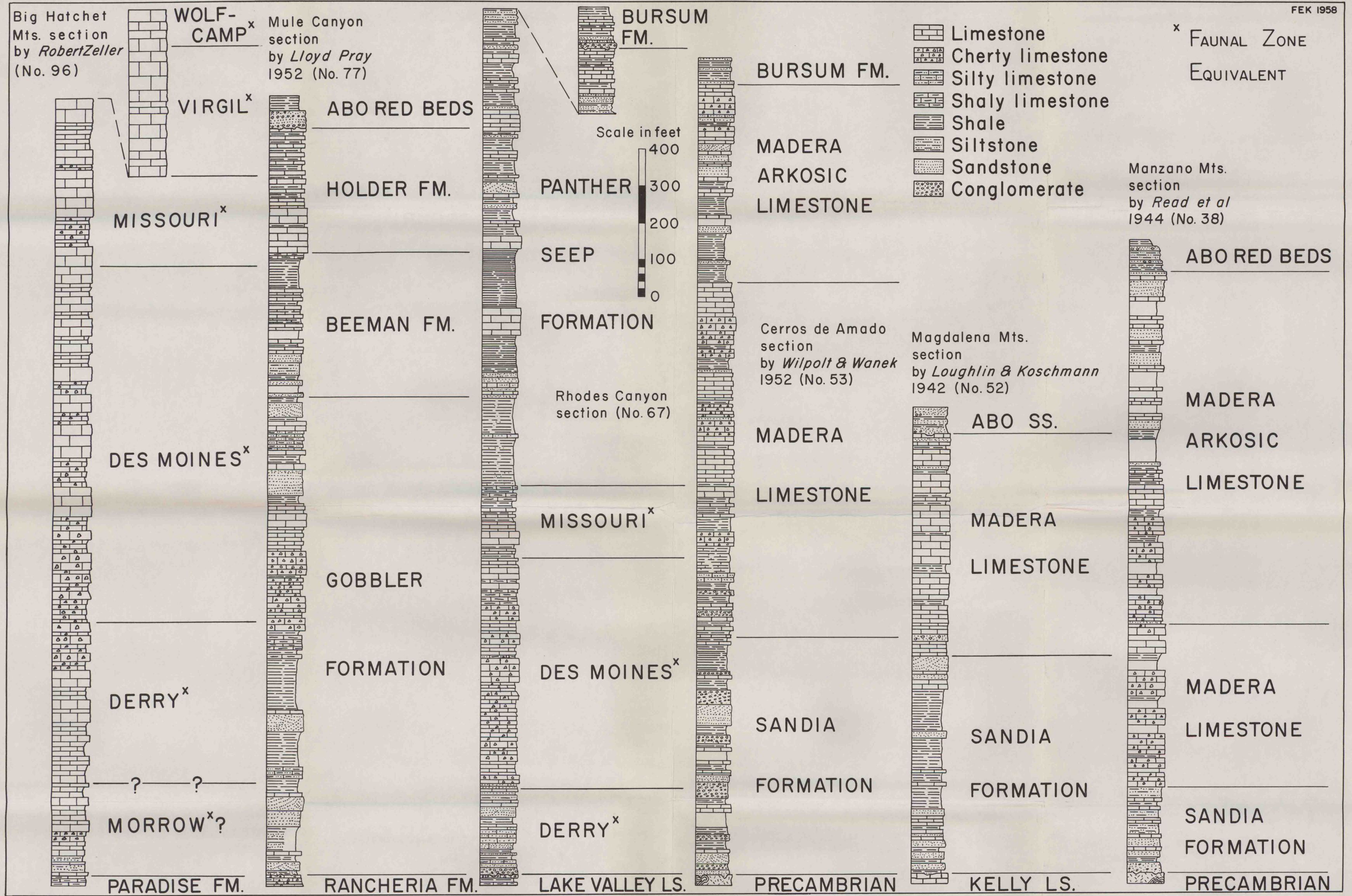
KEY COLUMNAR SECTIONS OF PENNSYLVANIAN ROCKS IN SOUTHWESTERN NEW MEXICO
