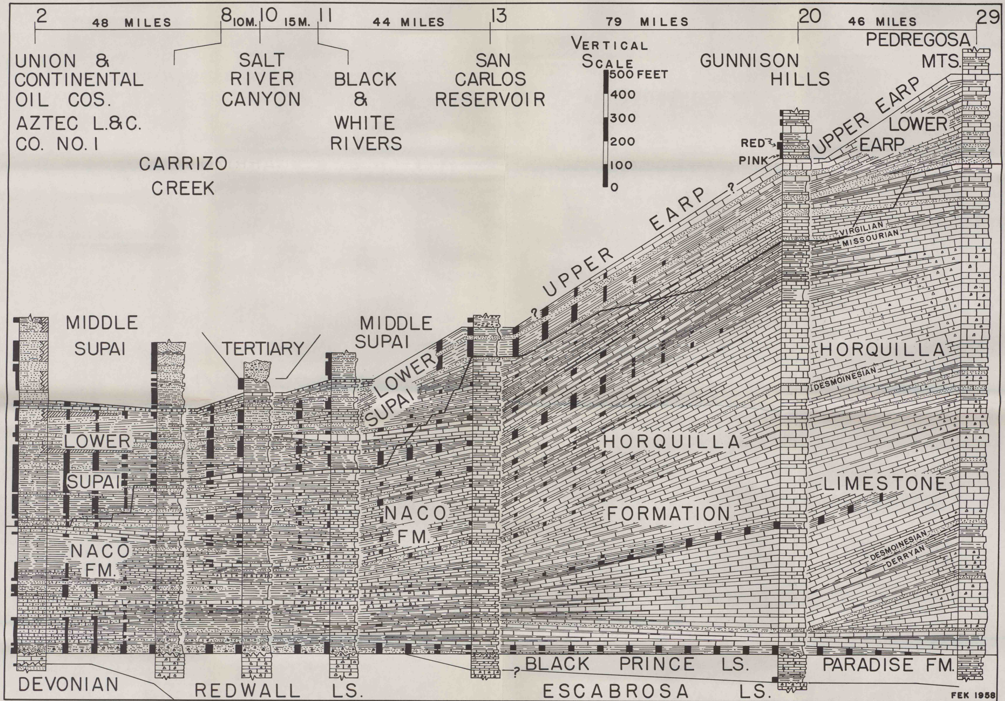
DIAGRAMMATIC SECTION FROM HOLBROOK ANTICLINE SOUTH-SOUTHEAST TO PEDREGOSA MOUNTAINS
