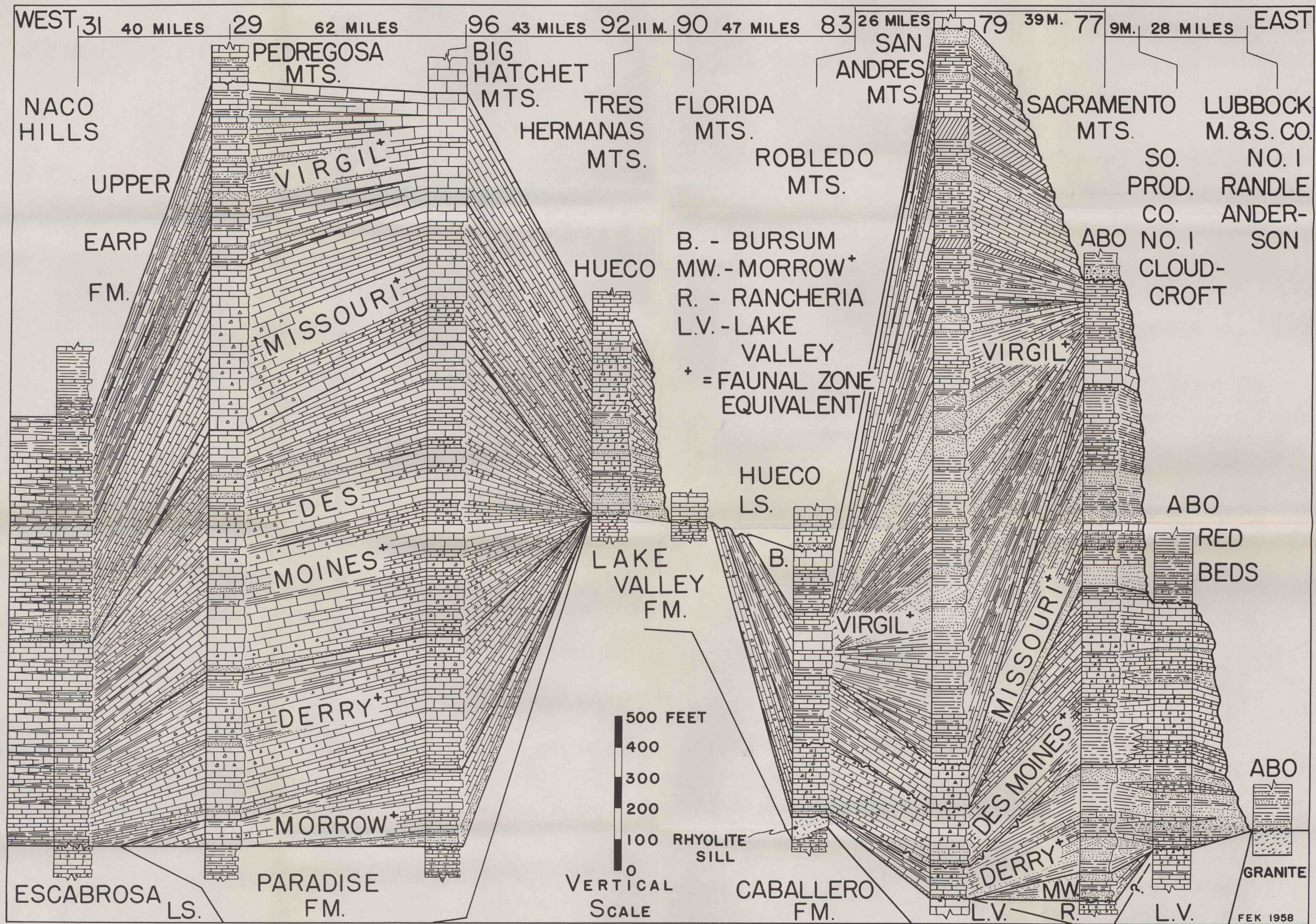
DIAGRAMMATIC SECTION FROM SACRAMENTO MOUNTAINS AREA WEST-SOUTHWESTWARD TO NACO HILLS
