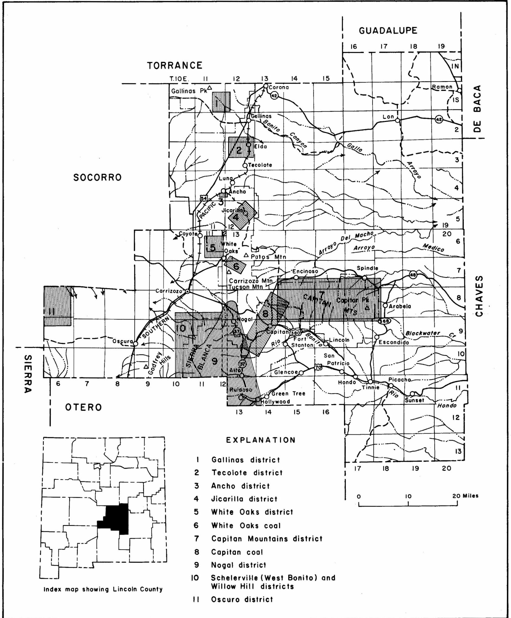
LOCATION MAP OF MINING DISTRICTS IN LINCOLN COUNTY
