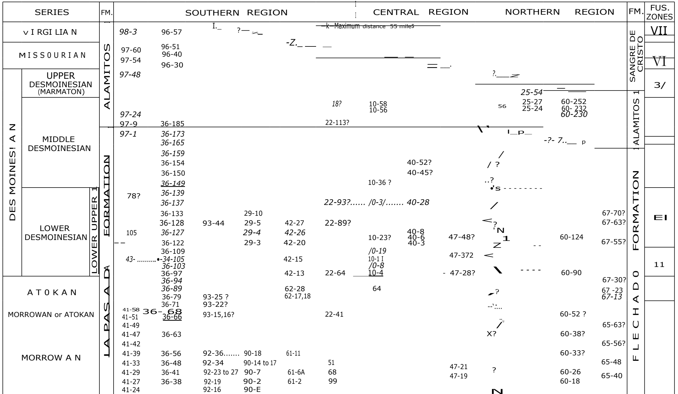
Figure 8. CORRELATION OF FOSSILIFEROUS UNITS
